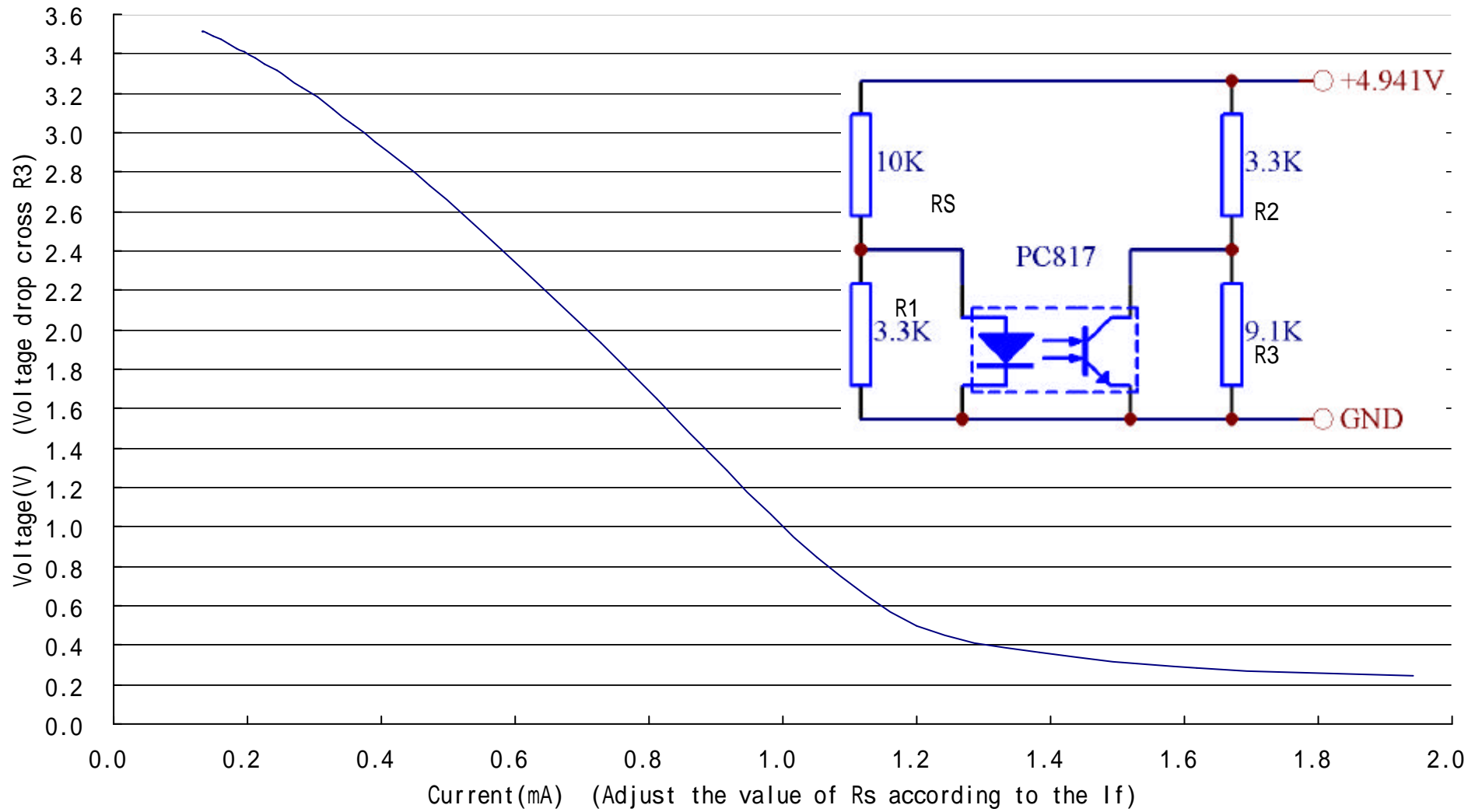
Input current vs Output voltage
