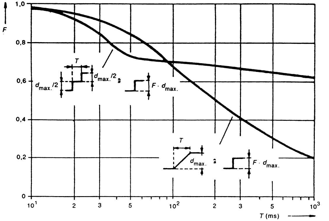
Figure 5 — Shape factors F for double-step and ramp-voltage characteristics
