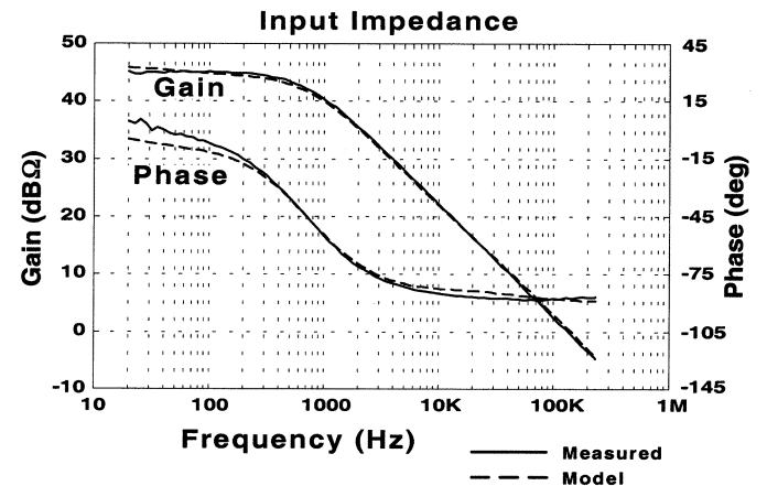
Fig. 17. PSPWM converter input impedance: measured result and small-signal model. Includes 1.2\text{ }\mu\text{F} input capacitance.
