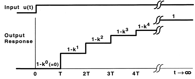
Fig. 9. Graph of input, u(t) , and piecewise constant staircase response.
