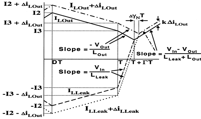
Fig. 4. Steady-state and perturbed currents ( V_{in} , V_{out} , D unperturbed).
