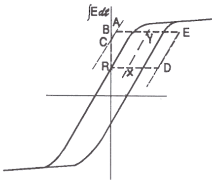
Fig 11. - Forward Converter Core Flux, I_M
