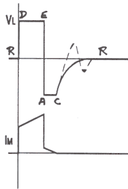
Fig 12. - Forward Converter Waveforms
