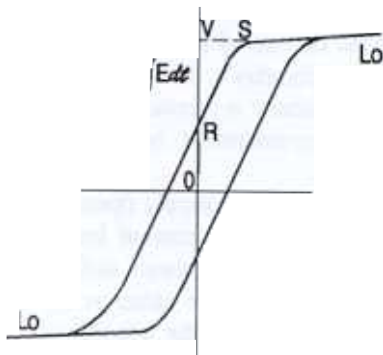
Fig 7. - Non-Homogeneous Effects
