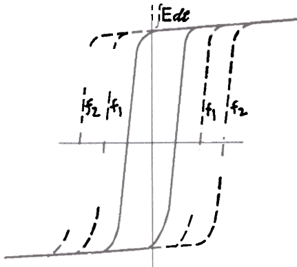
Fig 10. - L.F. Hysteresis plus Eddy Current
