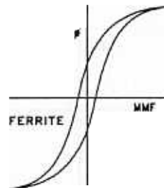
Fig 2. - Core Flux vs. Magnetic Force
