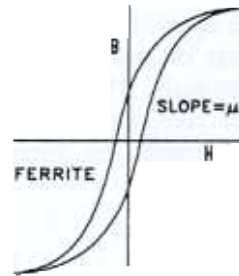
Fig 1. - Magnetic Core B-H Characteristic
