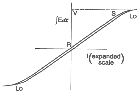
Fig 8. - Large Air Gap
