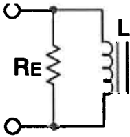
Fig 9. - Core Eddy Current Model
