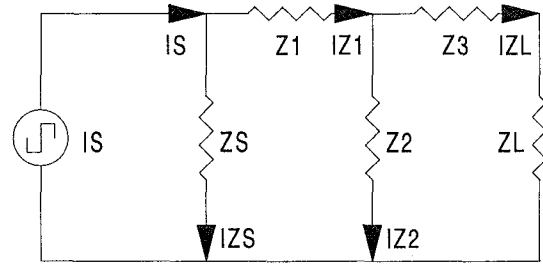
Fig. 5 - Current-Fed T-filter converter
