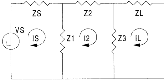
Fig. 1 - Voltage Fed \pi -filter converter
