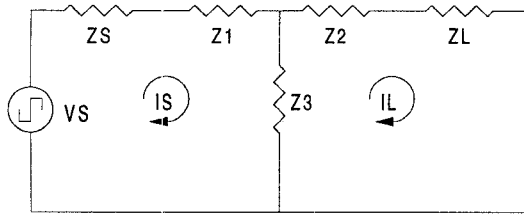
Fig. 3 - Voltage fed T-filter converter
