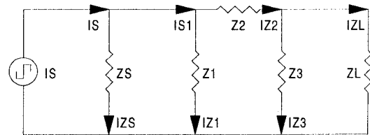
Fig 4 - Current-Fed \pi -filter converter
