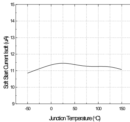
Figure 14. Soft Start Current
