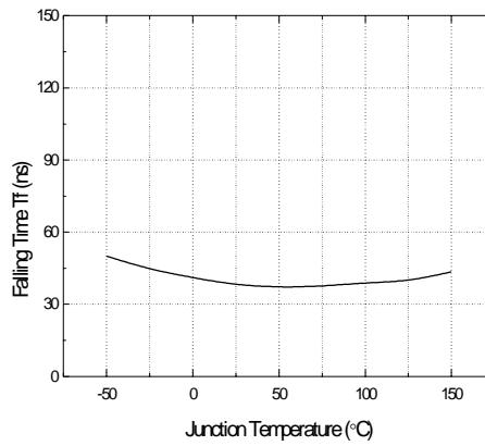
Figure 10. Output Falling Time
