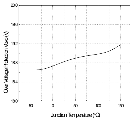
Figure 12. Over Voltage Protection Level
