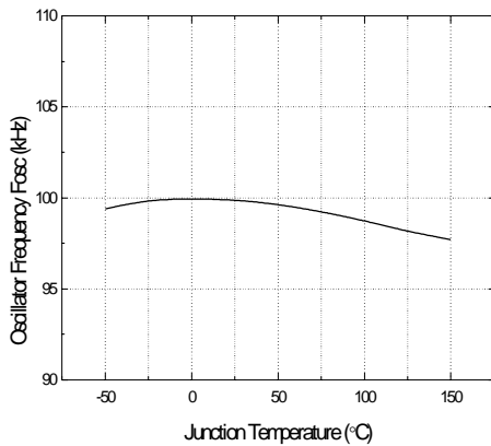
Figure 5. Oscillator Frequency
