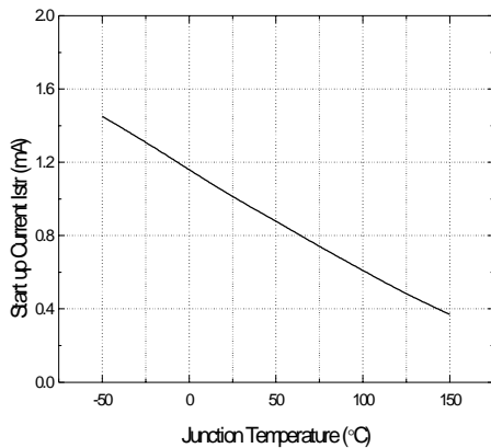
Figure 11. Start-up Current
