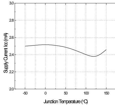
Figure 2. Supply Current
