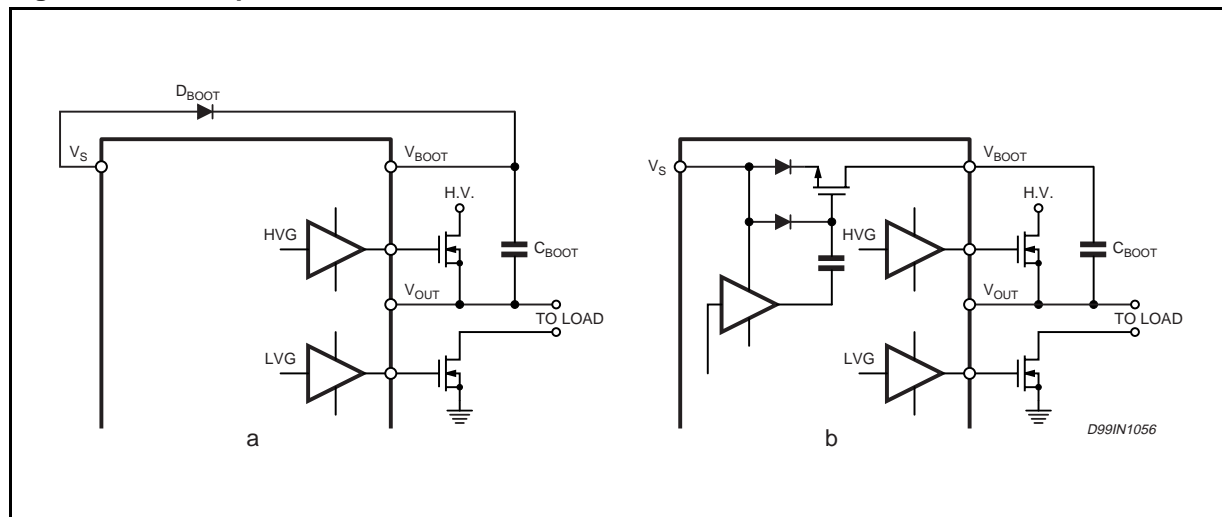
Figure 8. Bootstrap Driver
