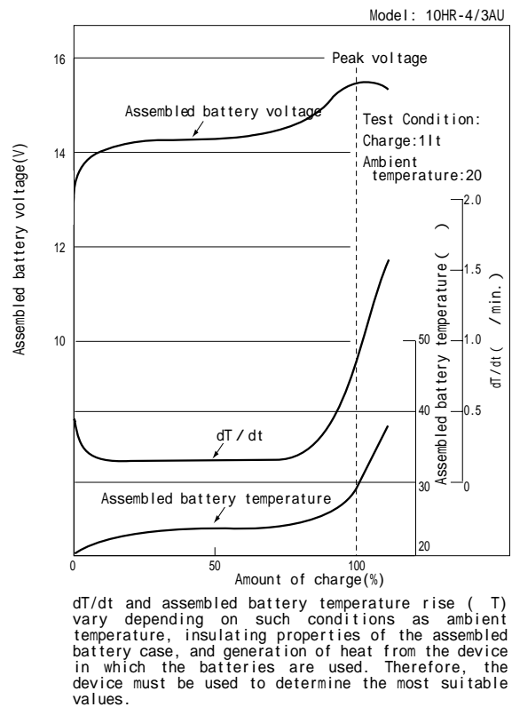
Fig.21 Quick charge control methods
