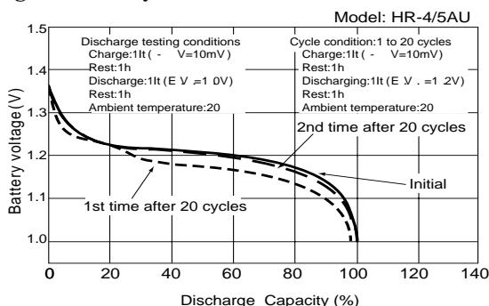
Fig. 18 Memory effect
