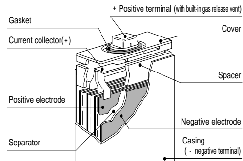
Fig.5 Internal structure of the Twicell SLIM
