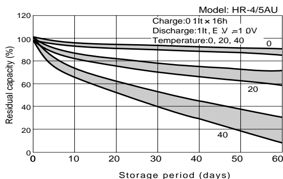
Fig.13 Storage characteristics
