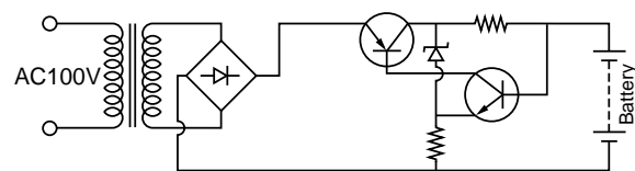
Fig.19 Example of a constant current charging circuit
