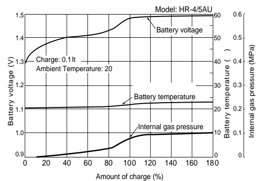
Fig.6 Charge characteristics
