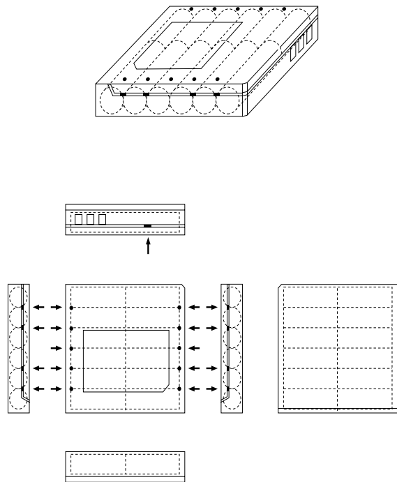
Fig.25 Cylindrical assembled battery: 2 x 6HR-AU
