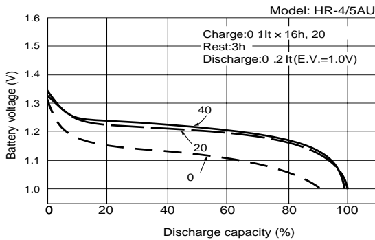
Fig.11 Discharge temperature characteristics
