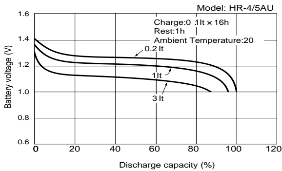
Fig.10 Discharge voltage characteristics
