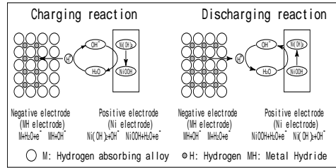
Fig. 3 Mechanism of the charging/discharging reaction of the nickel-metal hydride battery
