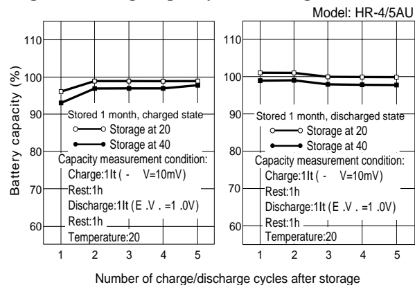
Fig.14 Discharge capacity after storage
