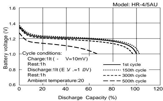
Fig.17 Discharge voltage and charge/discharge cycles
