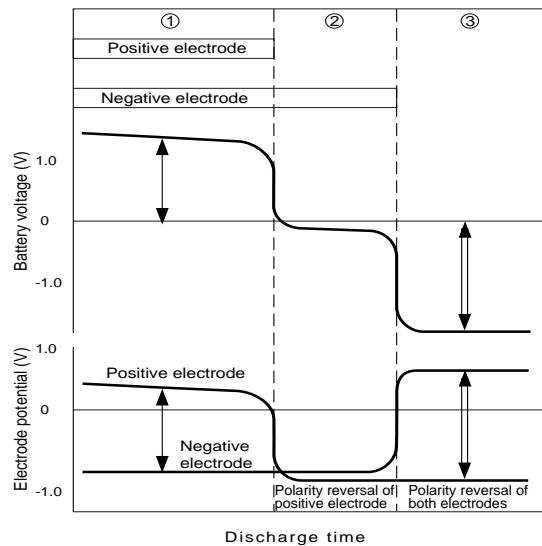
Fig.12 Polarity reversal
