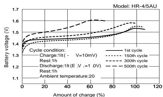
Fig.16 Charge characteristics and charge/discharge cycles
