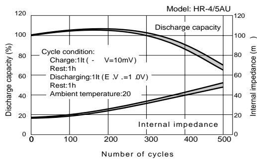
Fig.15 Charge/discharge cycle characteristics
