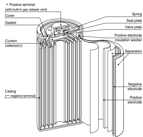
Fig.4 Internal structure of the Twicell
