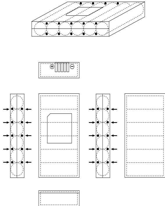
Fig.24 Cylindrical assembled battery: 6HR-AU
