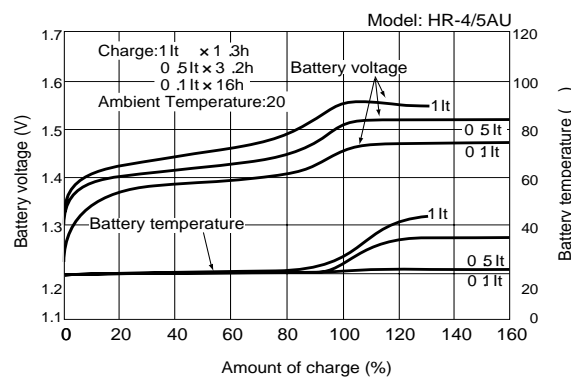
Fig.8 Charge temperature characteristics
