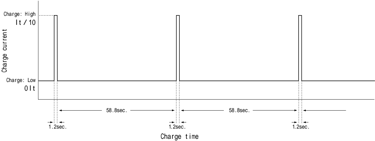
Fig. 22 Trickle charge by pulse current
