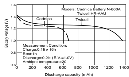
Fig. 1 Comparison of discharge capacities of Cadnica and Twicell.
