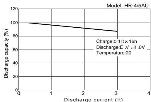
Fig.9 Discharge current and discharge capacity
