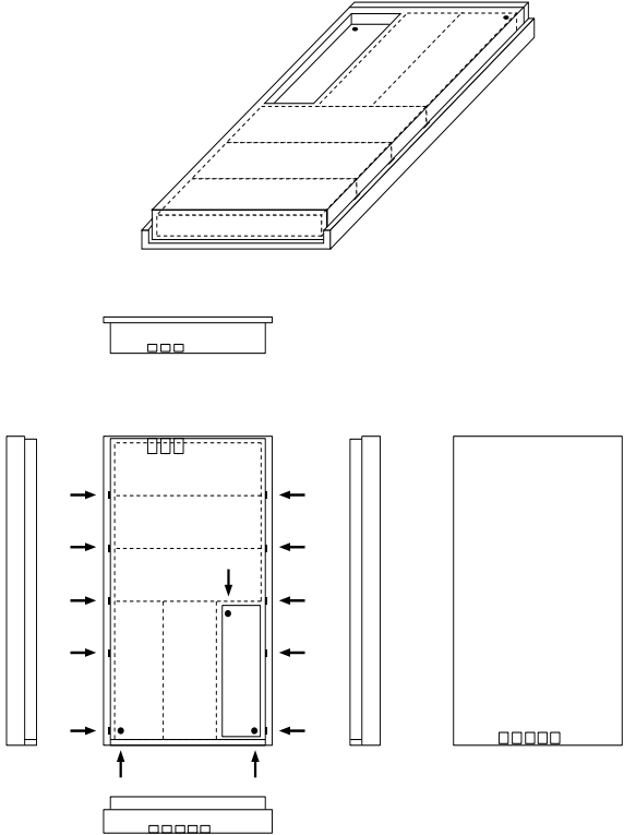
Fig.27 Rectangular assembled battery: 5HF-B1U
