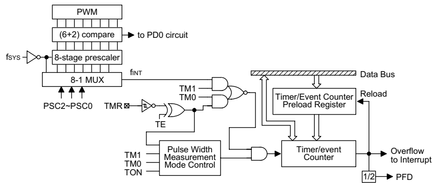
Timer/event counter
