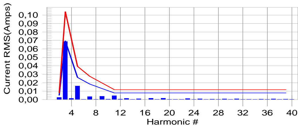
Diagramm: THD ClassC: Pmax=110W, Vinac=270V, Iout=140mA, Vaout=420V, PF=0.883
