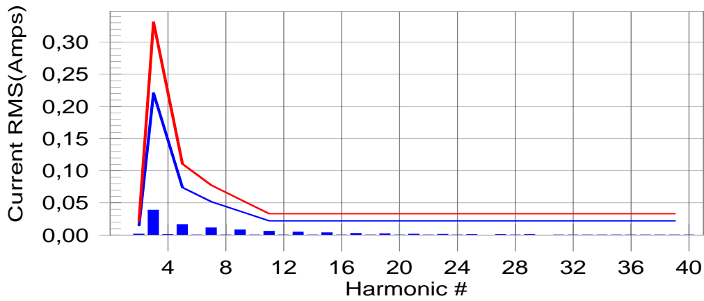
Diagramm: THD ClassC: Pmax=110W, Vinac=90V, Iout=140mA, Vaout=420V, PF=0.999
