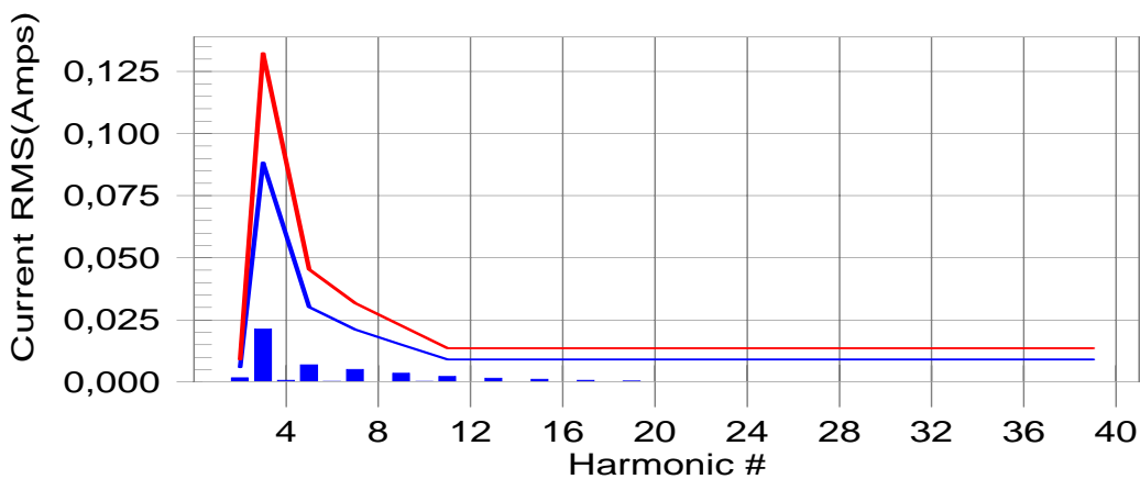
Diagramm: THD ClassC: Pmax=110W, Vinac=270V, Iout=140mA, Vaout=420V, PF=0.975
