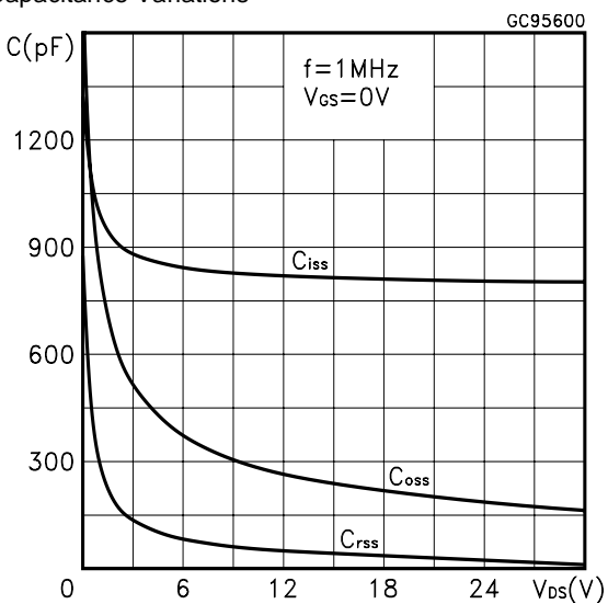
Capacitance Variations
