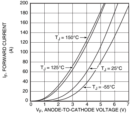
Figure 26. Forward Current vs. Forward Voltage
