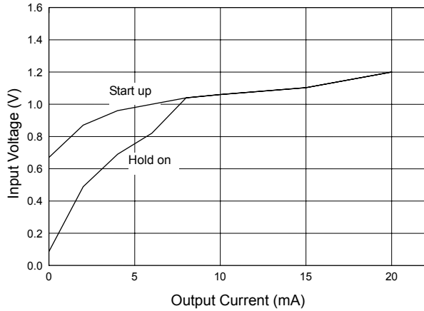
Fig. 40 AIC1642-37 Start-up & Hold-on Voltage (L=100 \mu H)
