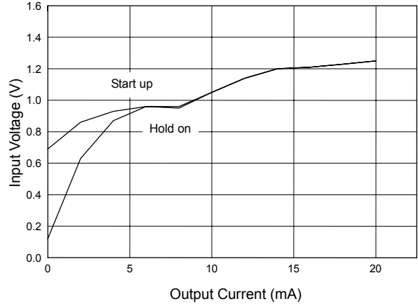
Fig. 47 AIC1642-45 Start-up & Hold-On Voltage (L=100 \mu H)
