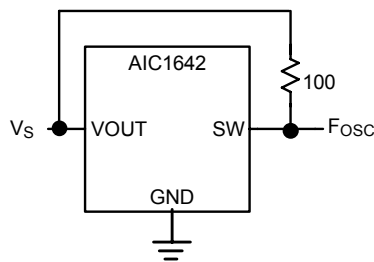
Fig. 3 Test Circuit 3
