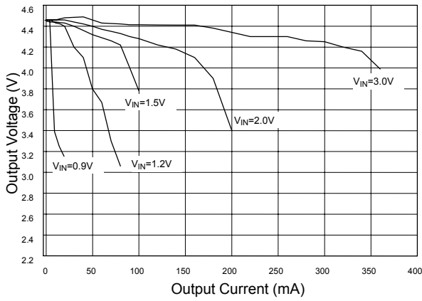
Fig. 46 AIC1642-45 Load Regulation (L=100 \mu H)
