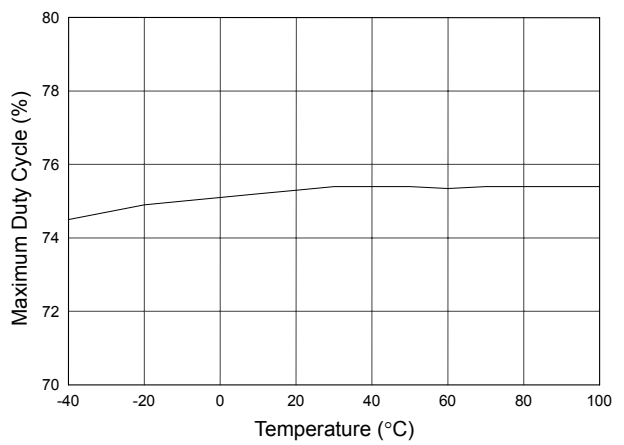
Fig. 51 AIC1642-45 Maximum Duty Cycle vs. Temperature
