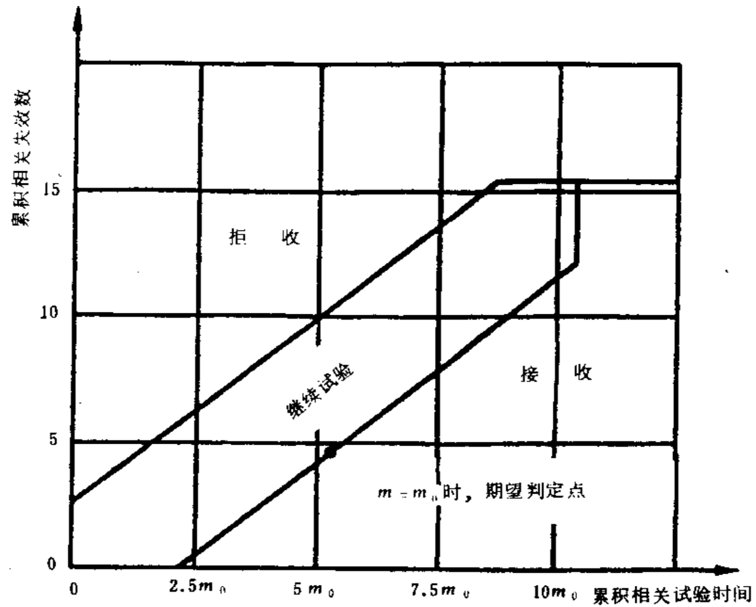
图 5 试验方案4:2 ( \alpha = 0.10, \beta = 0.10, D_m = 2.0 )
