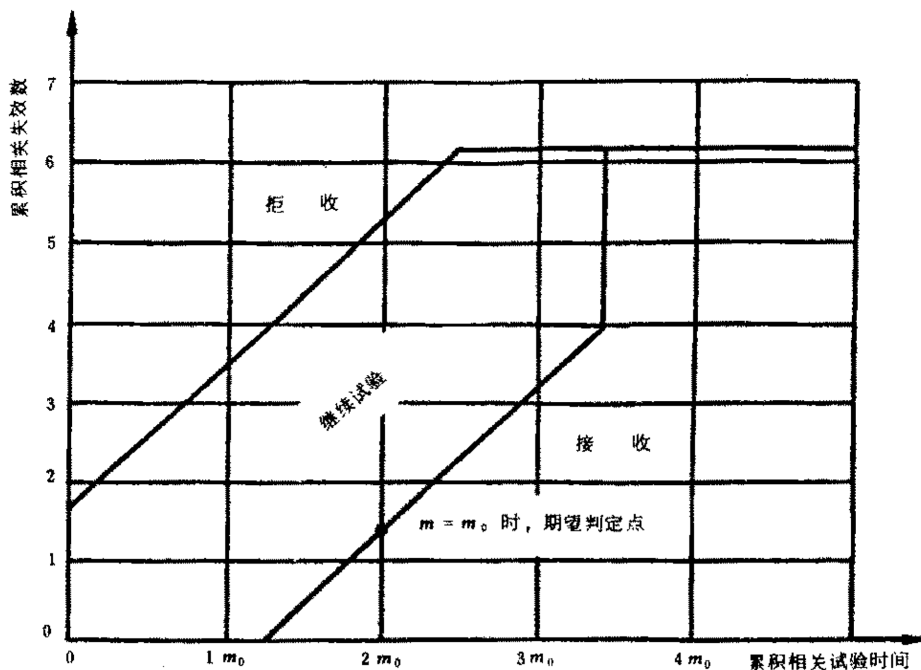
图 8 试验方案4:3 ( \alpha = 0.10, \beta = 0.10, D_m = 3.0 )
