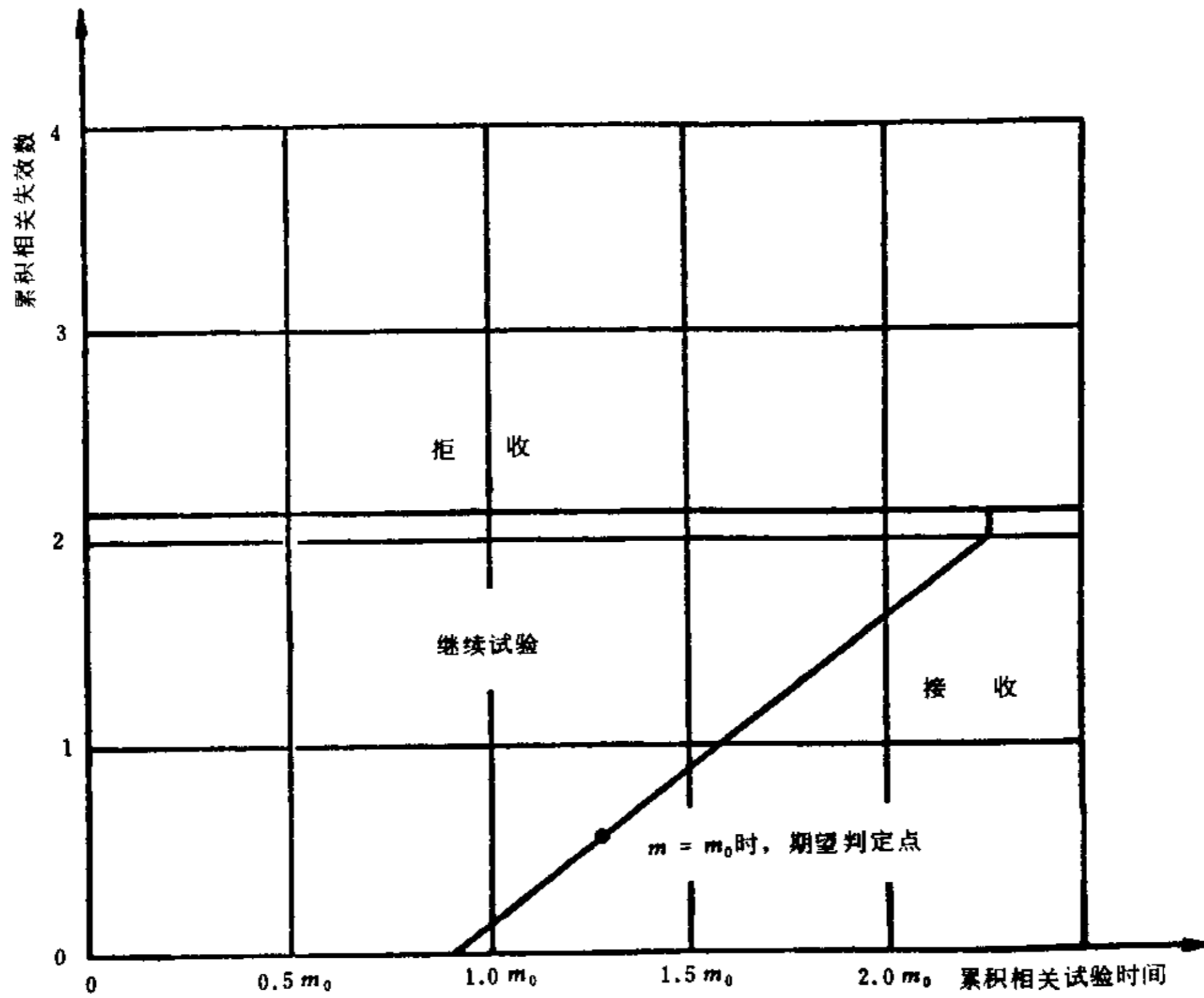
图 26 试验方案4:9 ( \alpha = 0.30, \beta = 0.30, D_m = 2.0 )
