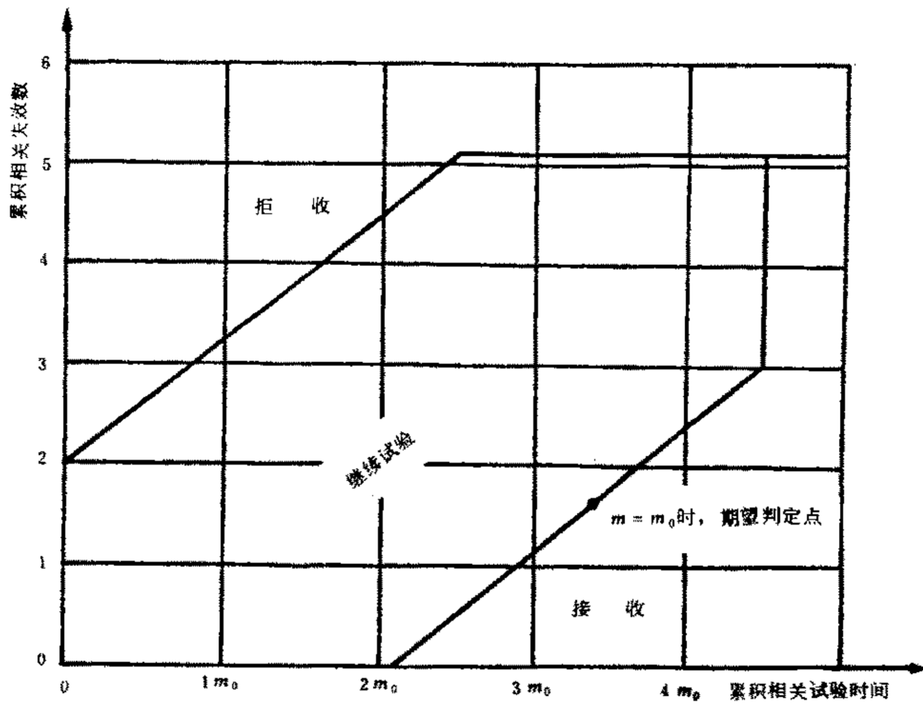
图 23 试验方案4:8 ( \alpha = 0.30, \beta = 0.30, D_m = 1.5 )
