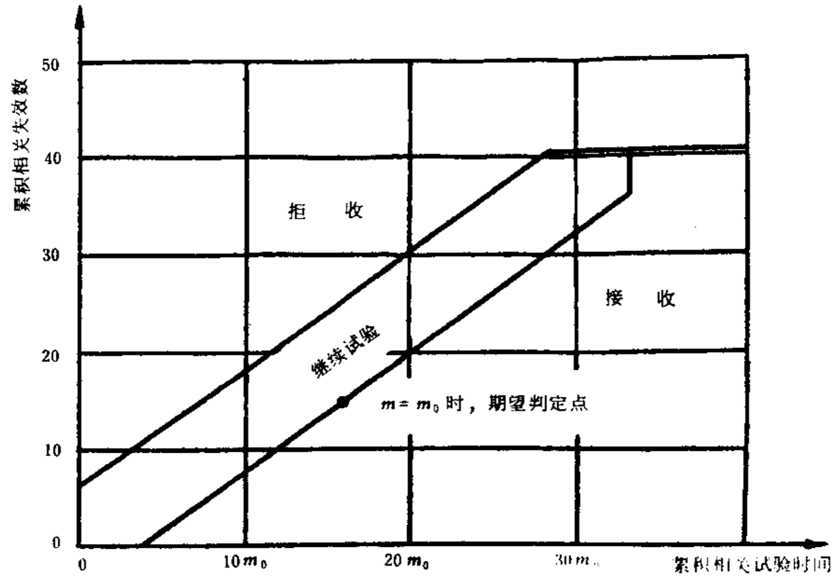
图 2 试验方案4:1 ( \alpha = 0.10, \beta = 0.10, D_m = 1.5 )
