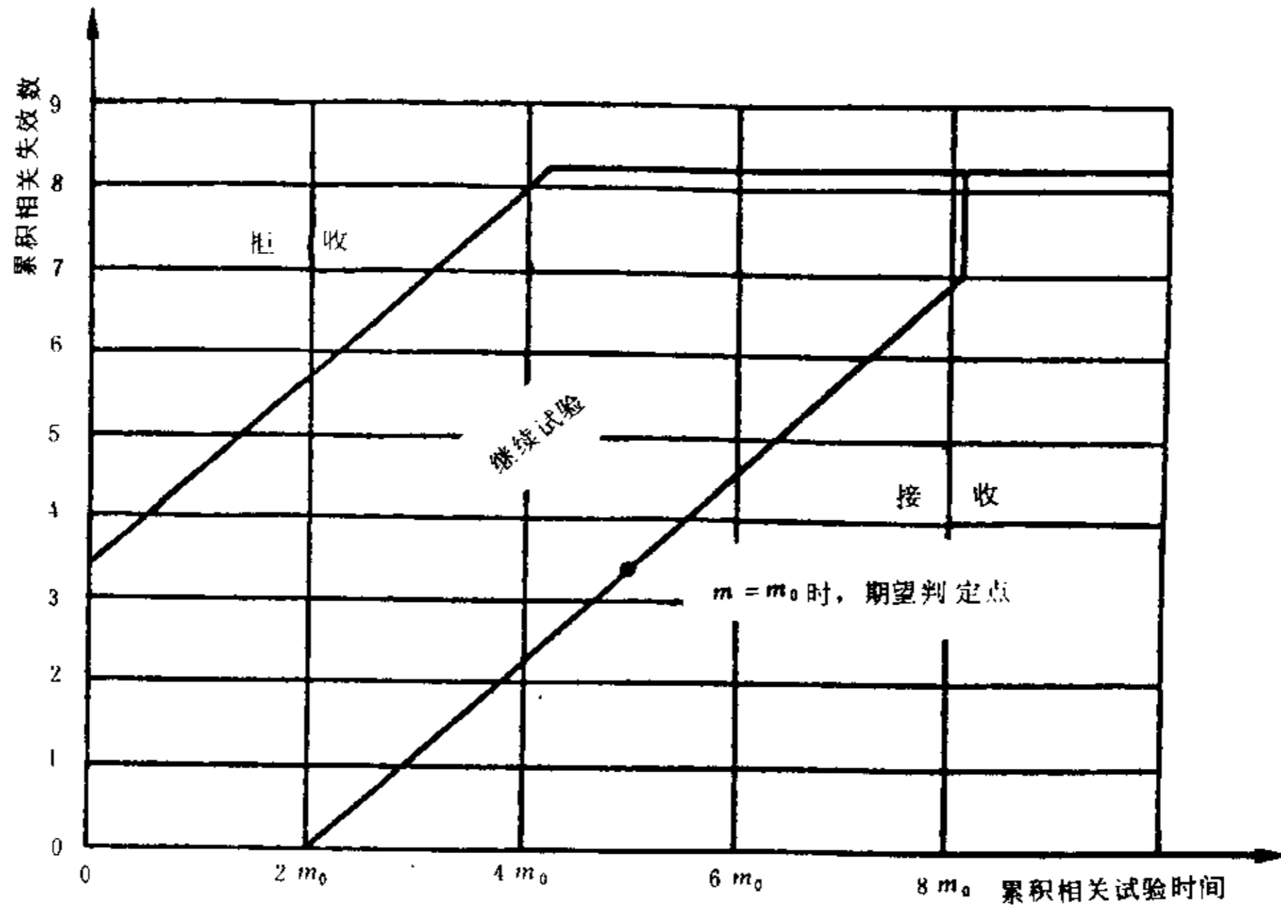
图 29 试验方案4:10 ( \alpha = 0.35, \beta = 0.40, D_m = 1.25 )
