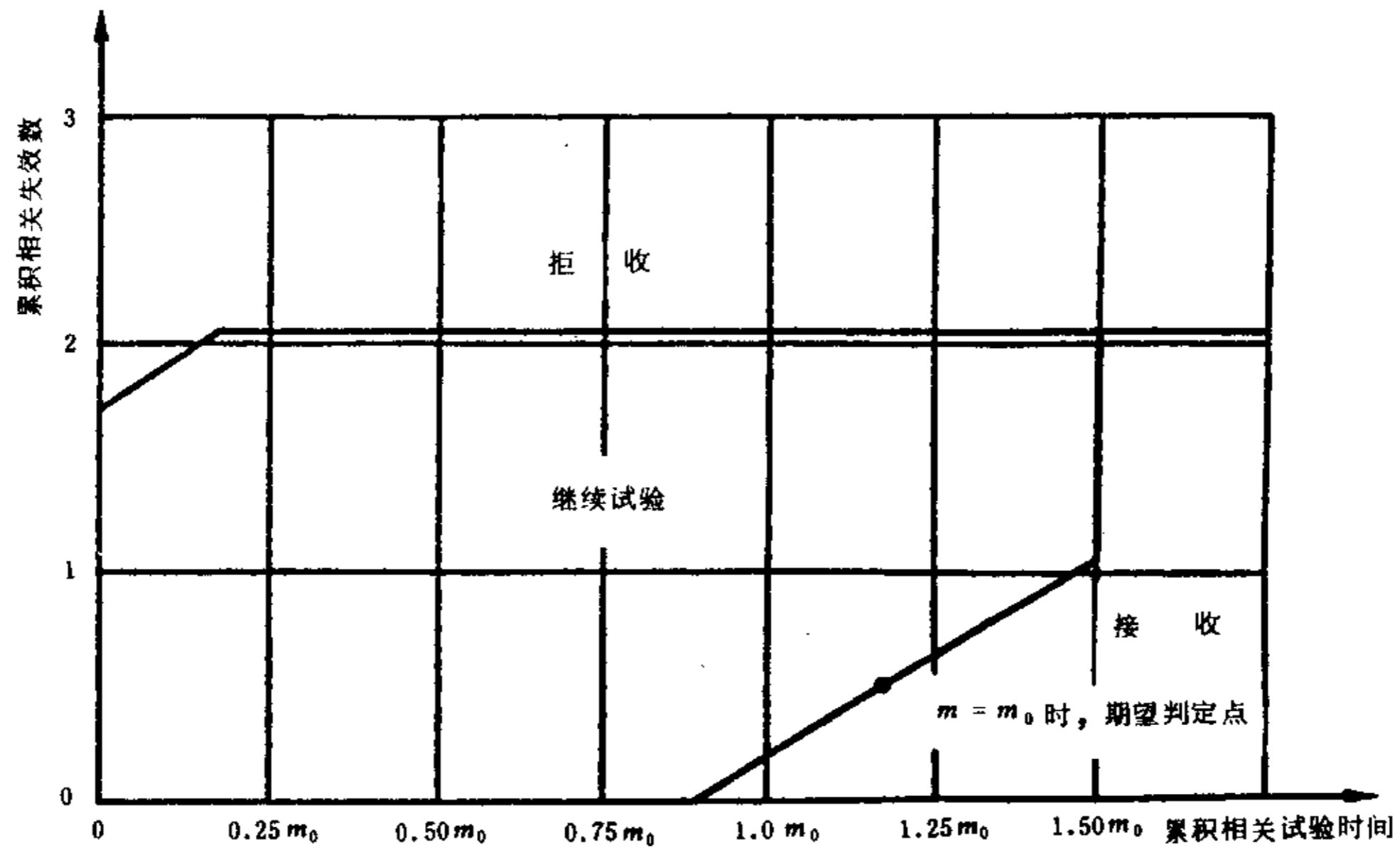
图 20 试验方案4:7 ( a = 0.20 , \beta = 0.20 , D_m = 3.0 )
