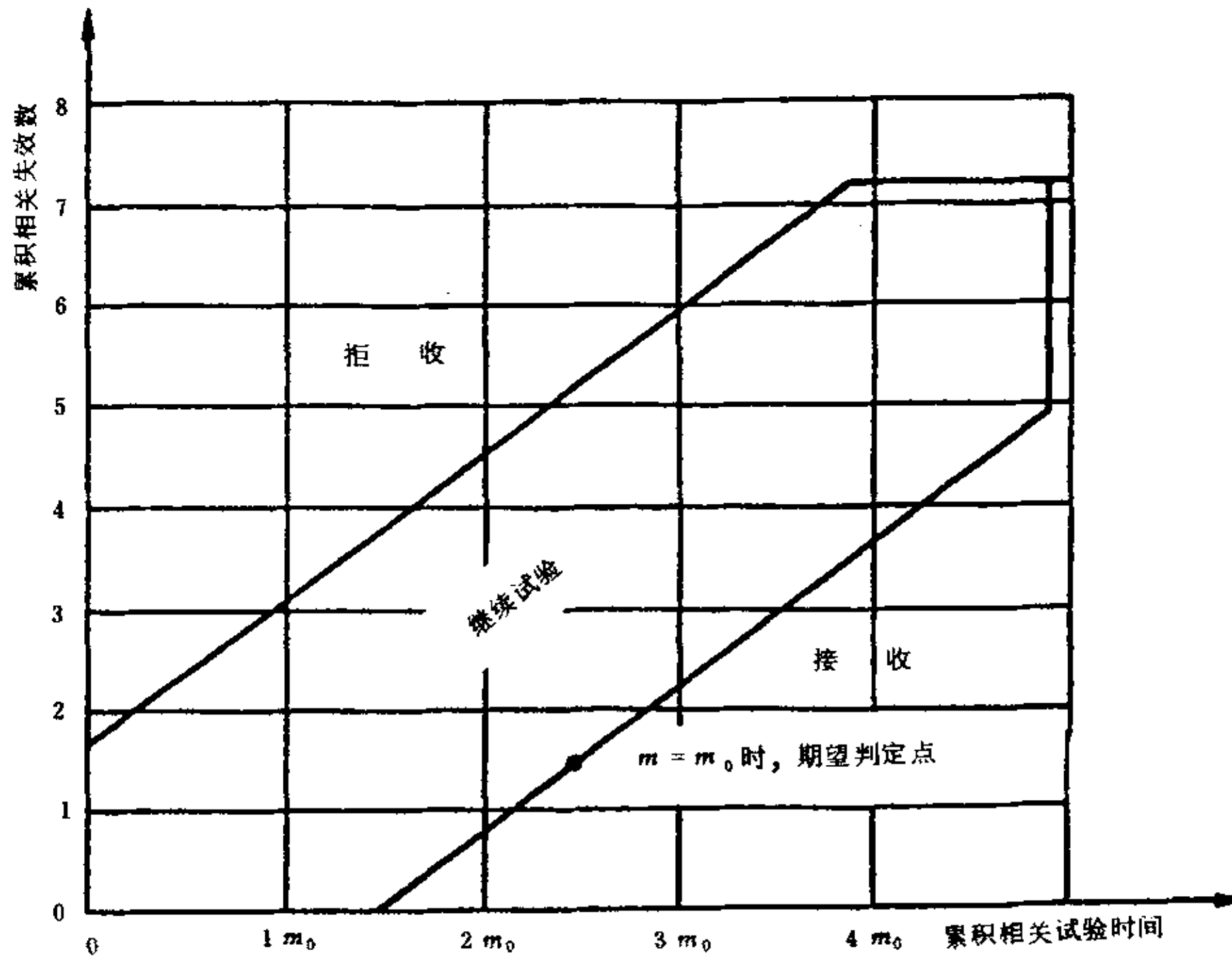
图 17 试验方案4:6 ( \alpha = 0.20 , \beta = 0.20 , D_m = 2.0 )
