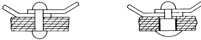
Figure 17 – Construction of electrical connections
