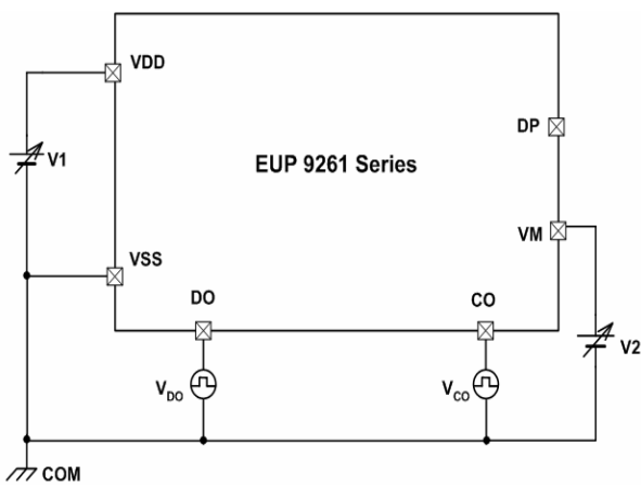
Measurement Circuit 5
