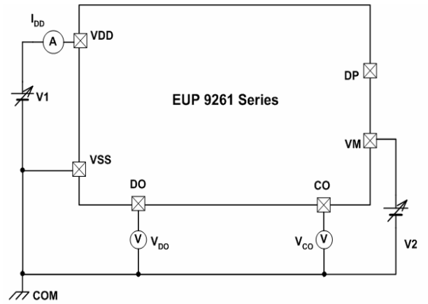
Measurement Circuit 2
