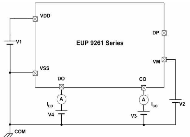
Measurement Circuit 4
