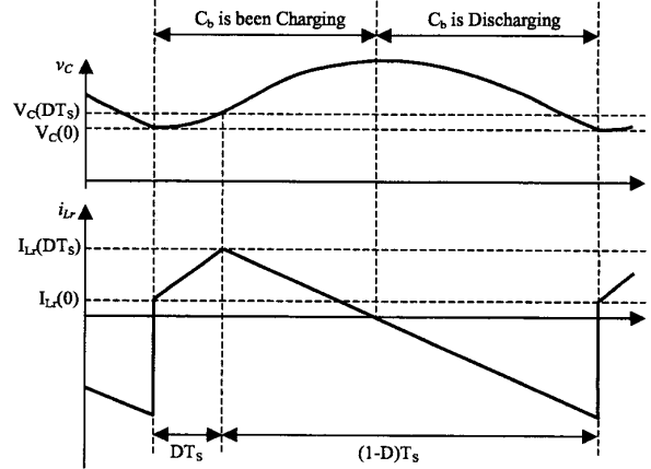
Fig. 4. Simplified waveforms of the voltage across the blocking capacitor and the current of the resonant inductor.
