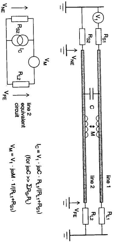
Figure 5.5 Superposition of inductive and capacitive coupling
