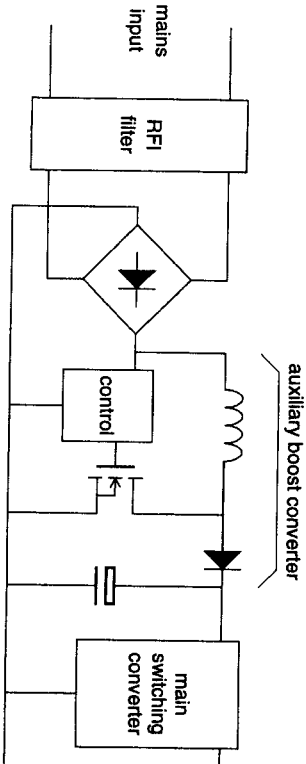
Figure 5.27 Schematic of a switchmode PFC circuit
