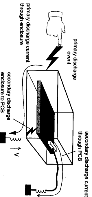
Figure 5.24 The cause of secondary discharge
