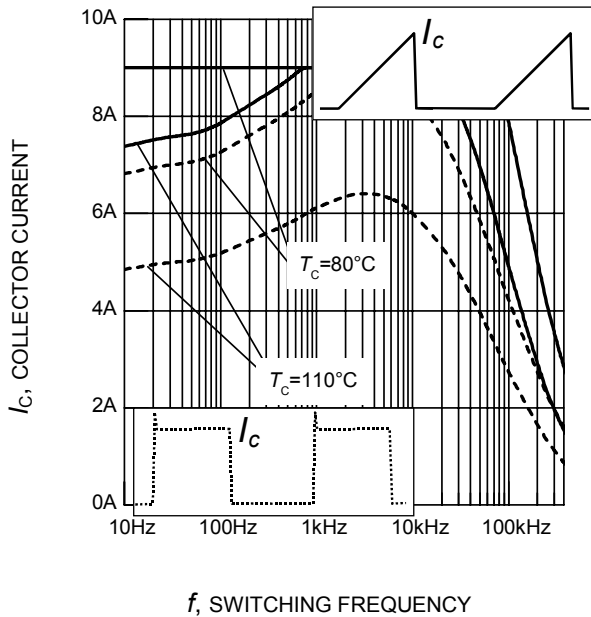
Figure 1. Collector current as a function of switching frequency ( T_j \leq 150^\circ\text{C} , D = 0.5 , V_{CE} = 400\text{V} , V_{GE} = 0/+15\text{V} , R_G = 80\Omega )
