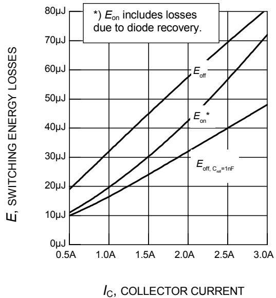
Figure 13. Typical switching energy losses as a function of collector current (inductive load, T_j = 150^\circ\text{C} , V_{CE} = 400\text{V} , V_{GE} = 0/+10\text{V} , R_G = 80\Omega , C = 0/1\text{nF} , Dynamic test circuit in Figure E)
