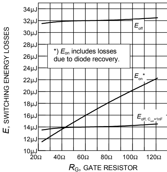
Figure 14. Typical switching energy losses as a function of gate resistor (inductive load, T_j = 150^\circ\text{C} , V_{CE} = 400\text{V} , V_{GE} = 0/+10\text{V} , I_C = 1\text{A} , Dynamic test circuit in Figure E)
