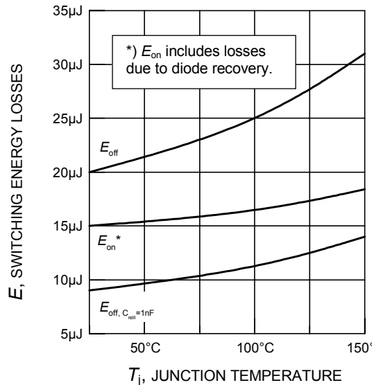
Figure 15. Typical switching energy losses as a function of junction temperature (inductive load, V_{CE} = 400\text{V} , V_{GE} = 0/+10\text{V} , I_C = 1\text{A} , R_G = 80\Omega , Dynamic test circuit in Figure E)
