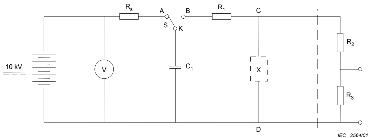
Figure 4 – Test hook
