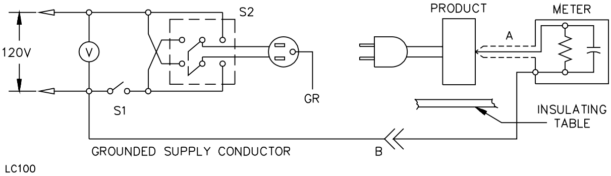
Figure 45.1 (47.1) Leakage-current measurement circuits
