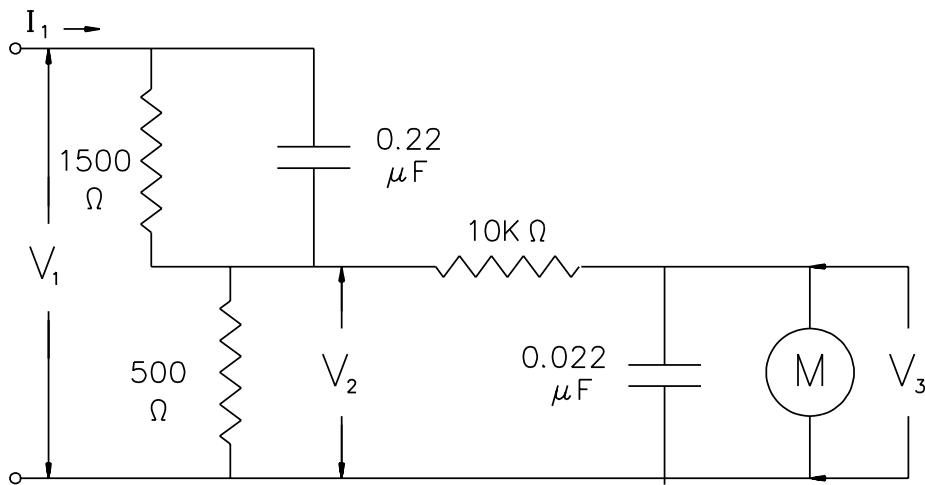
Figure 47.2 Measurement instrument for reaction (leakage) current
