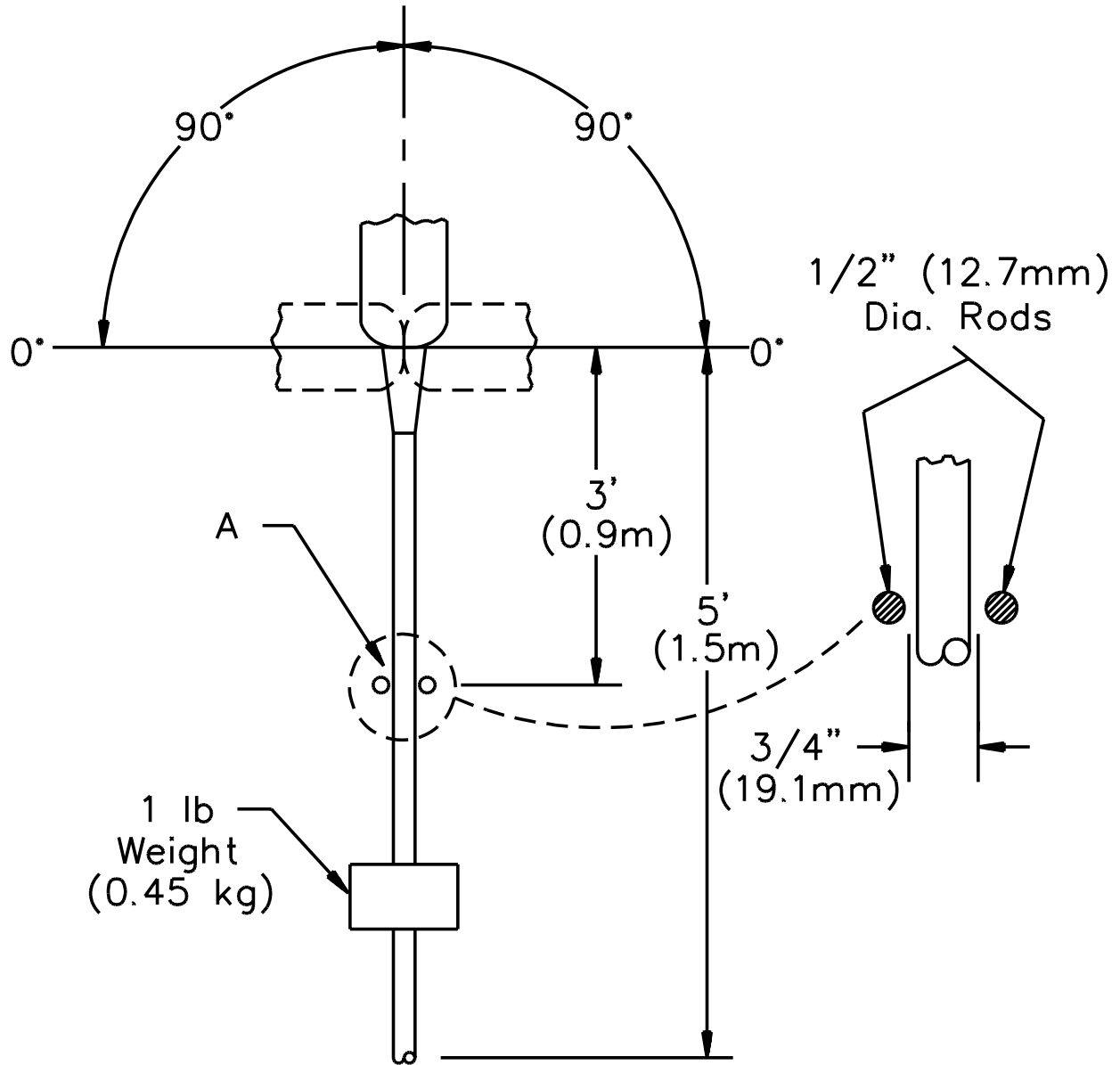
Figure 43.1 Cord flexing
