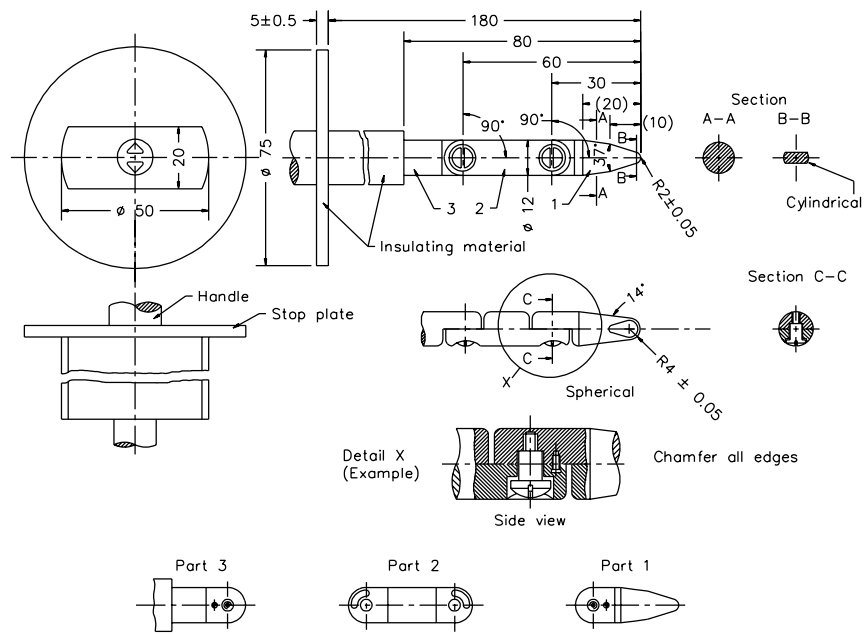
Figure 7.4 Articulate probe
