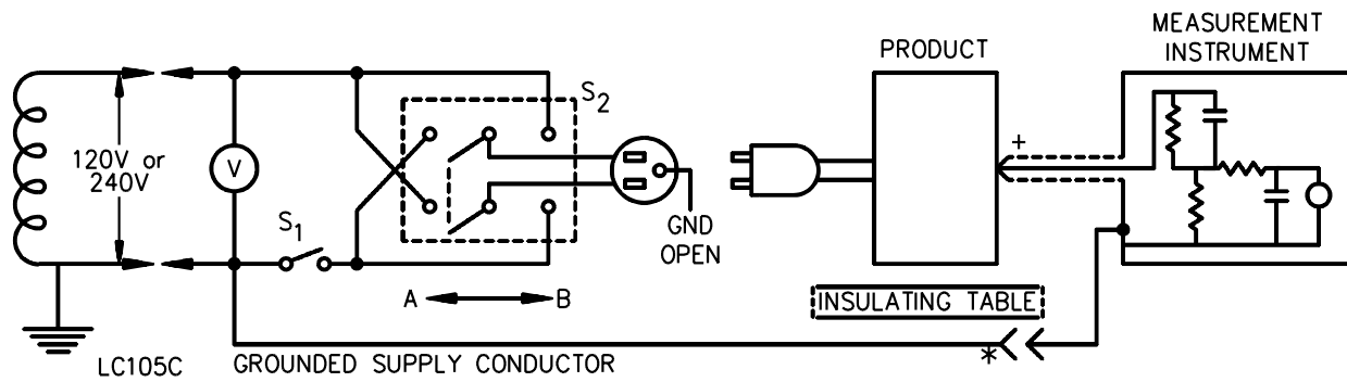
Figure 47.1 Typical leakage current measurement circuits
