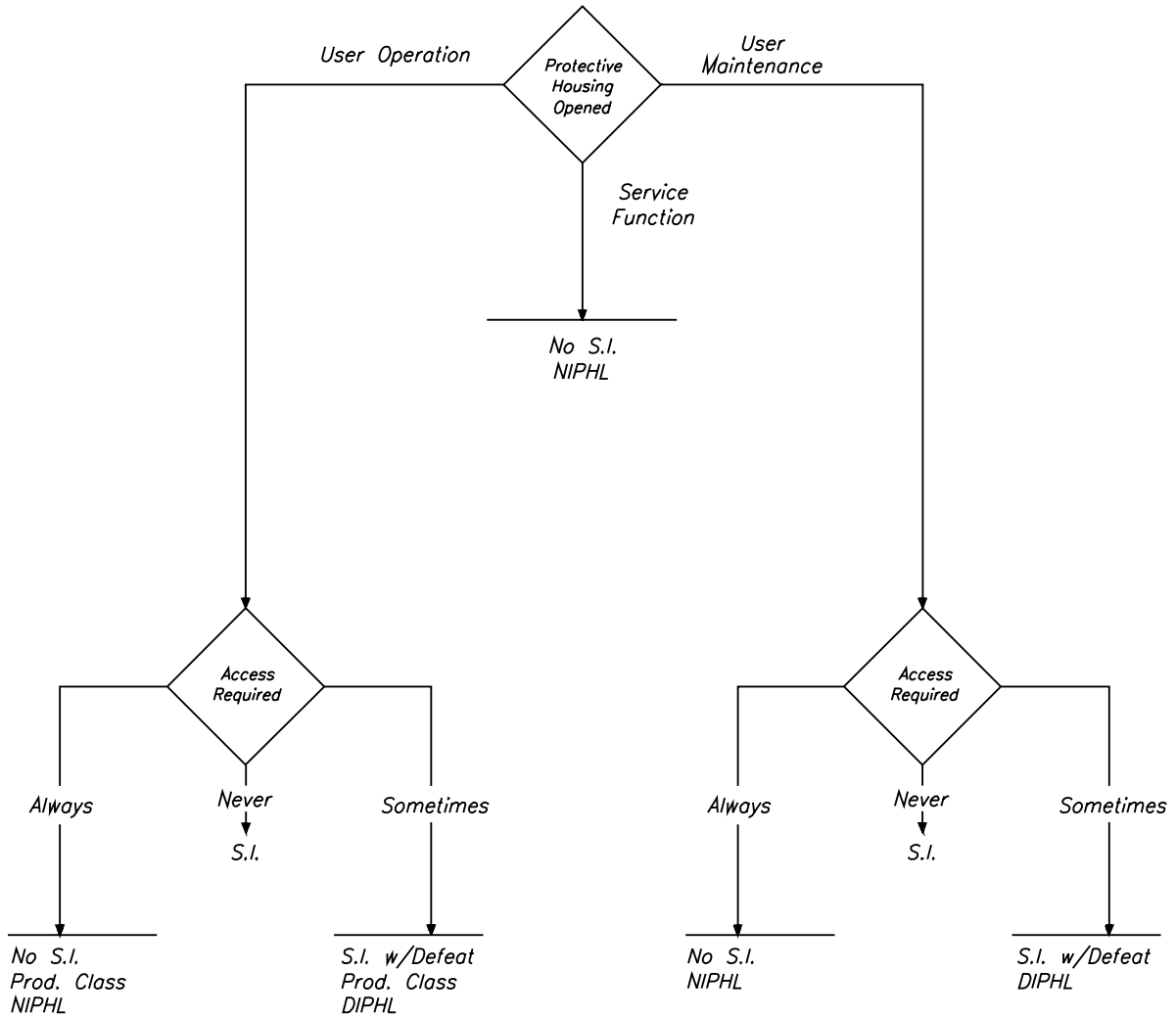
Figure 41.1 Laser product safety interlock requirements
