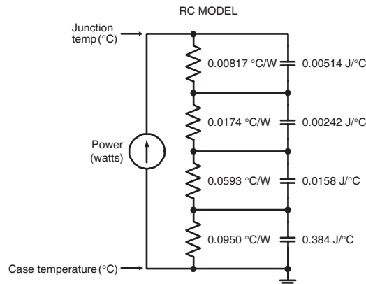
FIGURE 1b, TRANSIENT THERMAL IMPEDANCE MODEL
