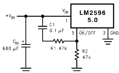
FIGURE 21. Delayed Startup
