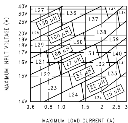
FIGURE 6. LM2596-12
