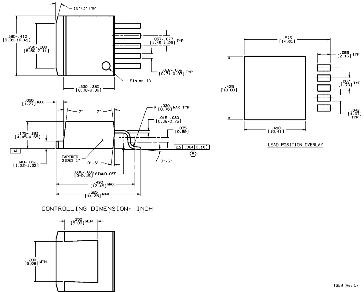
5-Lead TO-263 Surface Mount Package (S) Order Number LM2596S-3.3, LM2596S-5.0, LM2596S-12 or LM2596S-ADJ
