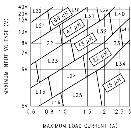
FIGURE 4. LM2596-3.3
