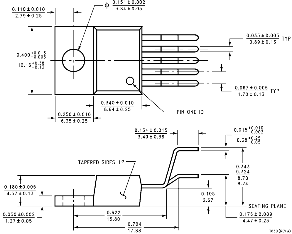
5-Lead TO-220 (T) Order Number LM2596T-3.3, LM2596T-5.0, LM2596T-12 or LM2596T-ADJ
