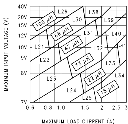
FIGURE 5. LM2596-5.0
