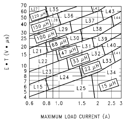
FIGURE 7. LM2596-ADJ
