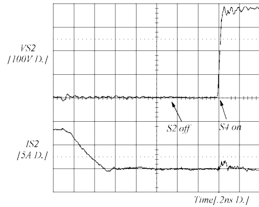
Fig. 11. ZCS waveforms of lagging-leg switches.
