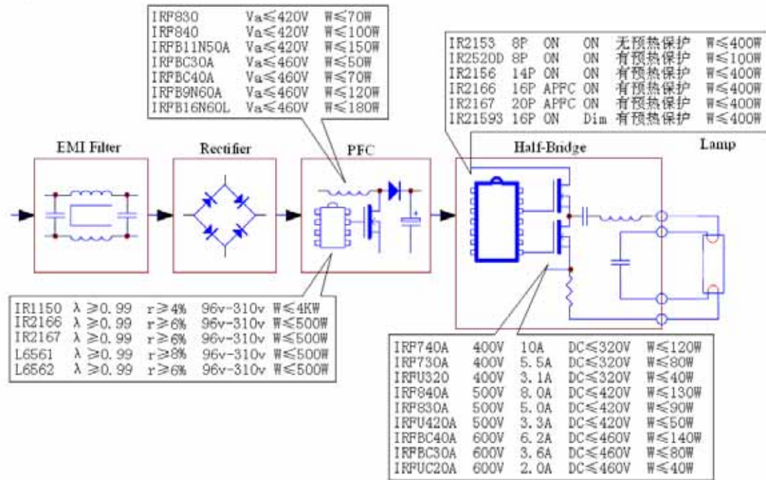
Fluorescent Lamp Ballast
