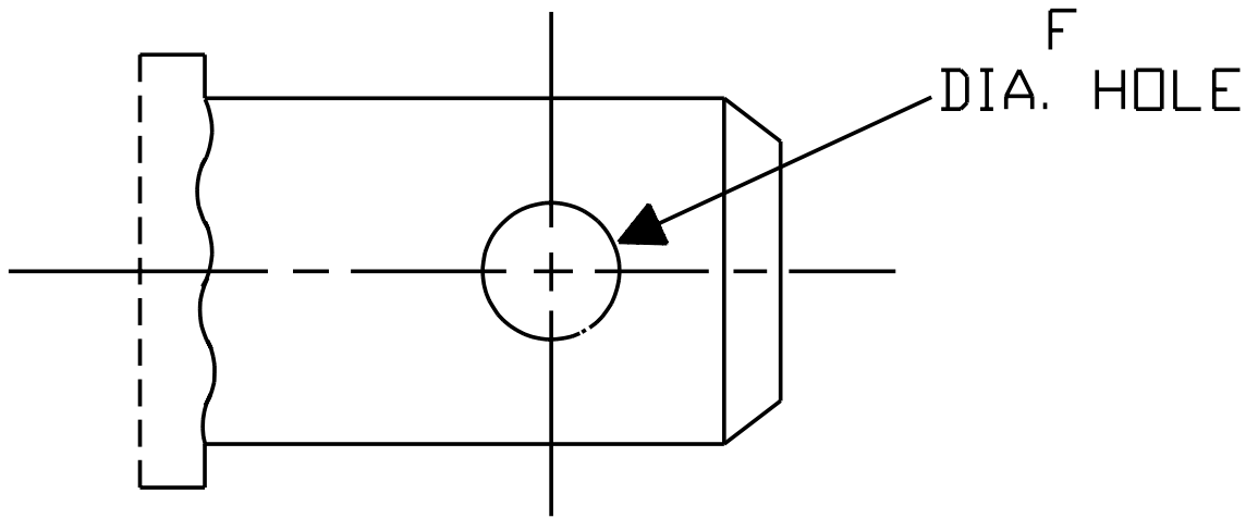
Figure 6.4 Dimensions of hole detents
