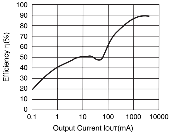
R1224N502G ( V_{IN}=16V )
