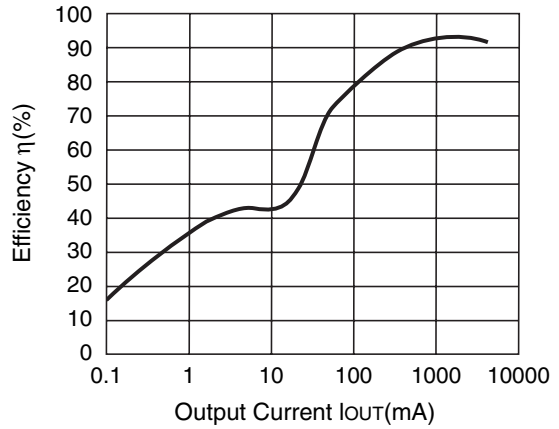
R1224N502G ( V_{IN}=10V )
