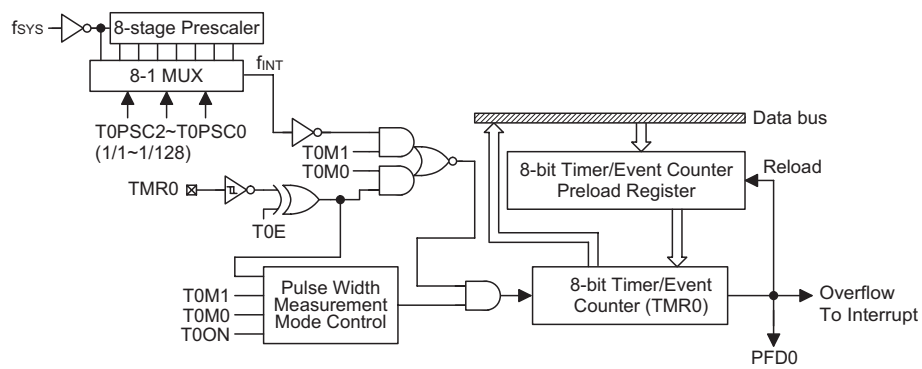
Timer/Event Counter 0
