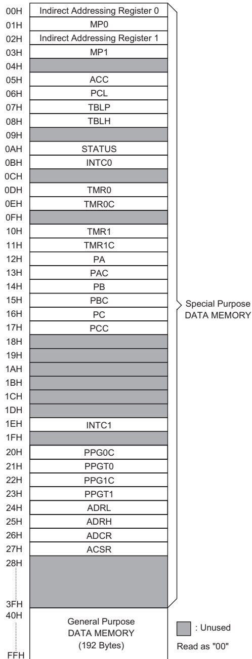
RAM Mapping
