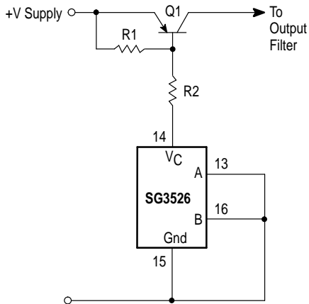
Figure 20. Single-Ended Configuration
