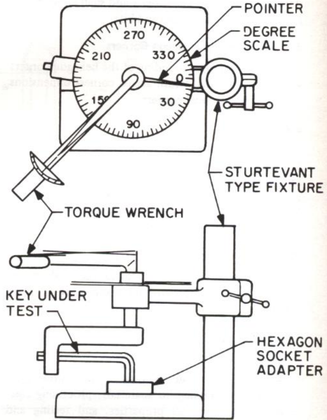
FIGURE 4. TYPICAL TORSIONAL STRENGTH TEST FIXTURE
