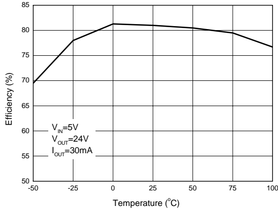
Figure 8. Efficiency vs. Temperature
