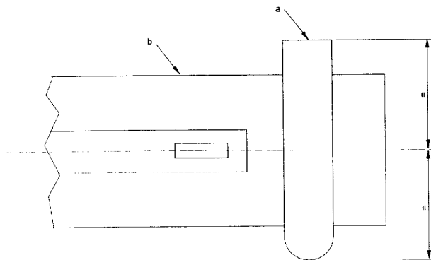
c) Plan view of guide plate showing position of test probe
