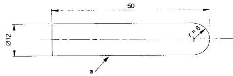
a) Details of test probe
