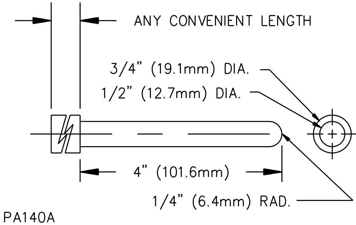
Figure 6.4 Probe for film-coated (magnet) wire
