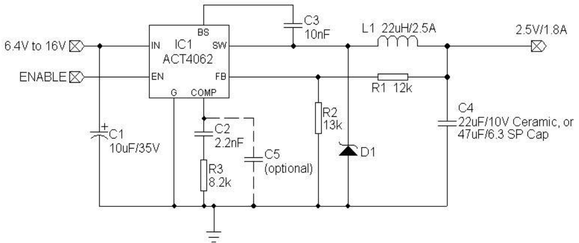
Figure 5. ACT4062 2.5V/1.8A Output Application
