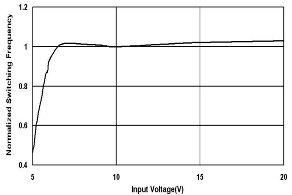
Normalized Switching Frequency vs. Input
