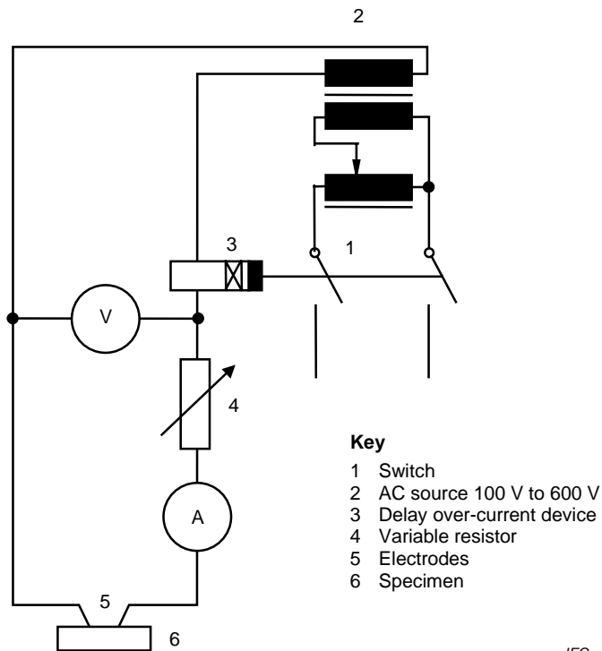
Figure B.4 – Example of test circuit
