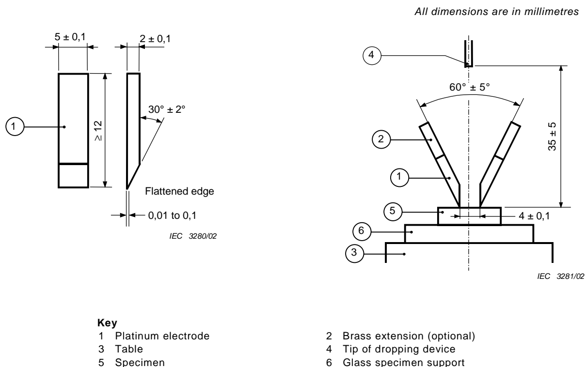
Figure B.1 – Electrode
