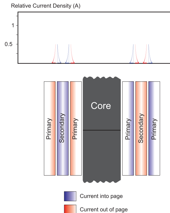
Figure 10: Current distribution with single-layer secondary and split primary transformer winding
