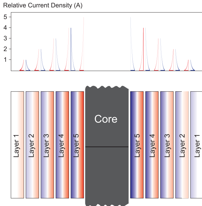
Figure 5: Current distribution with five-layer inductor winding
