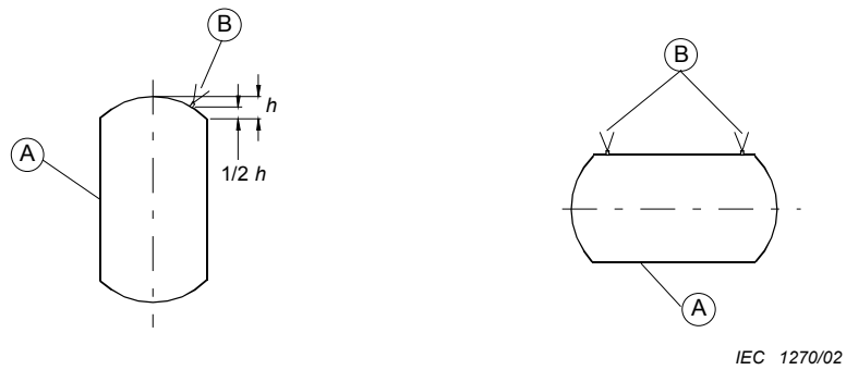
Figure 102a – Position of thermocouples for metallic containers
