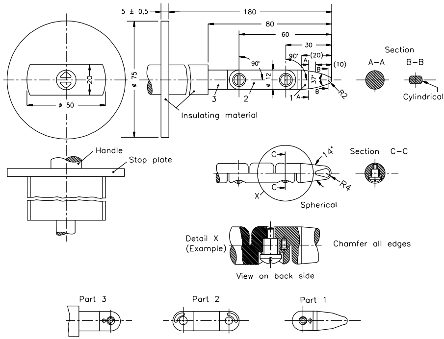
Linear dimensions in millimetres
