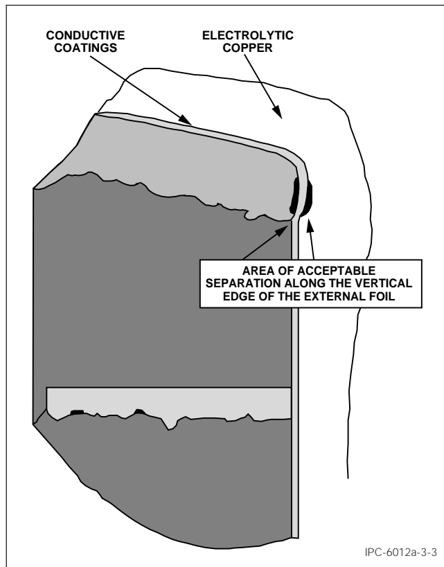
Figure 3-3 Separations at External Foil
