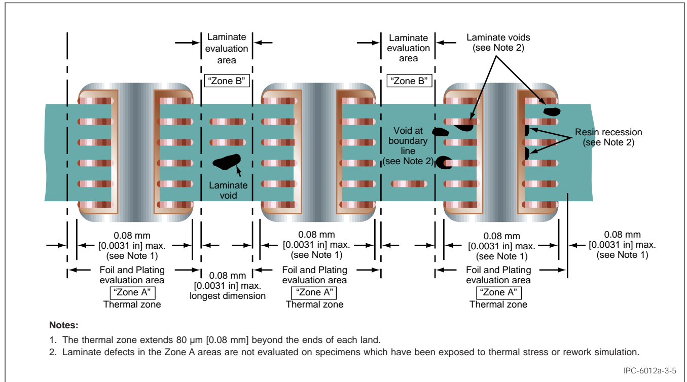
Figure 3-5 Typical Microsection Evaluation Specimen (Three Plated-Through Holes)
