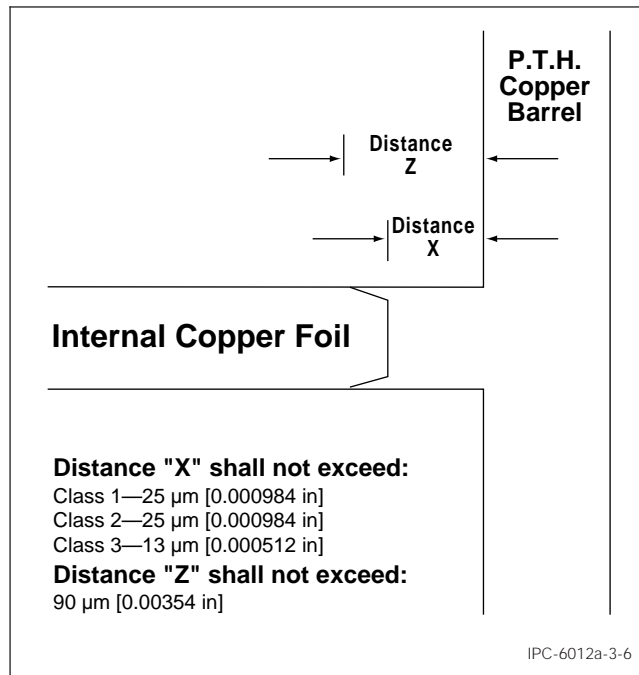
Figure 3-6 Negative Etchback
