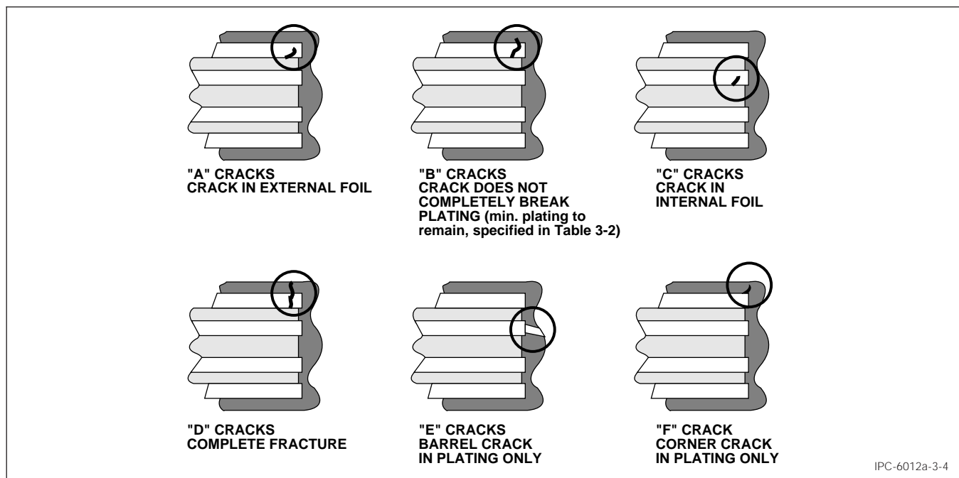
Figure 3-4 Crack Definition
