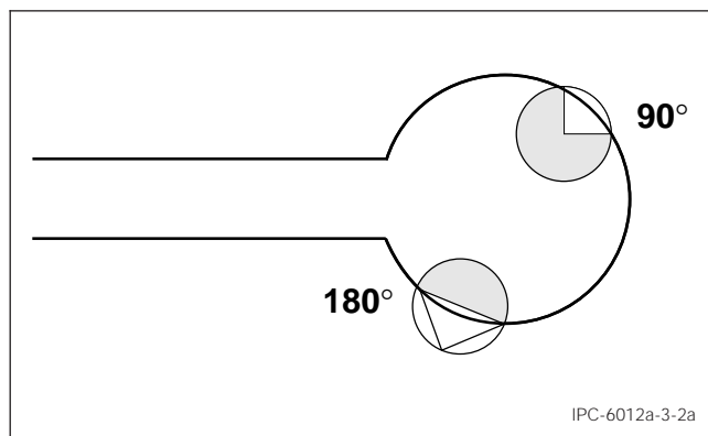
Figure 3-2A Breakout of 90° and 180°
