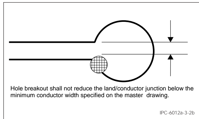
Figure 3-2B Conductor Width Reduction
