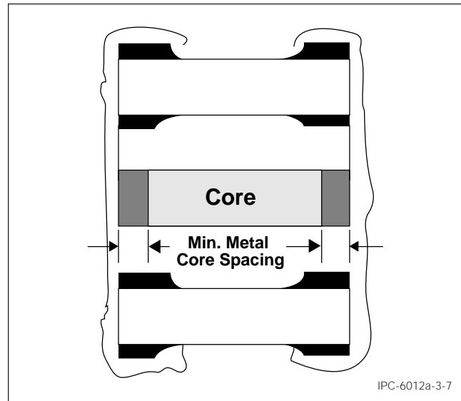
Figure 3-7 Metal Core to Plated-Through Hole Spacing
