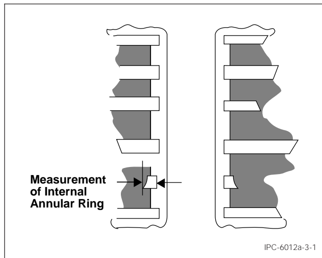
Figure 3-1 Annular Ring Measurement
