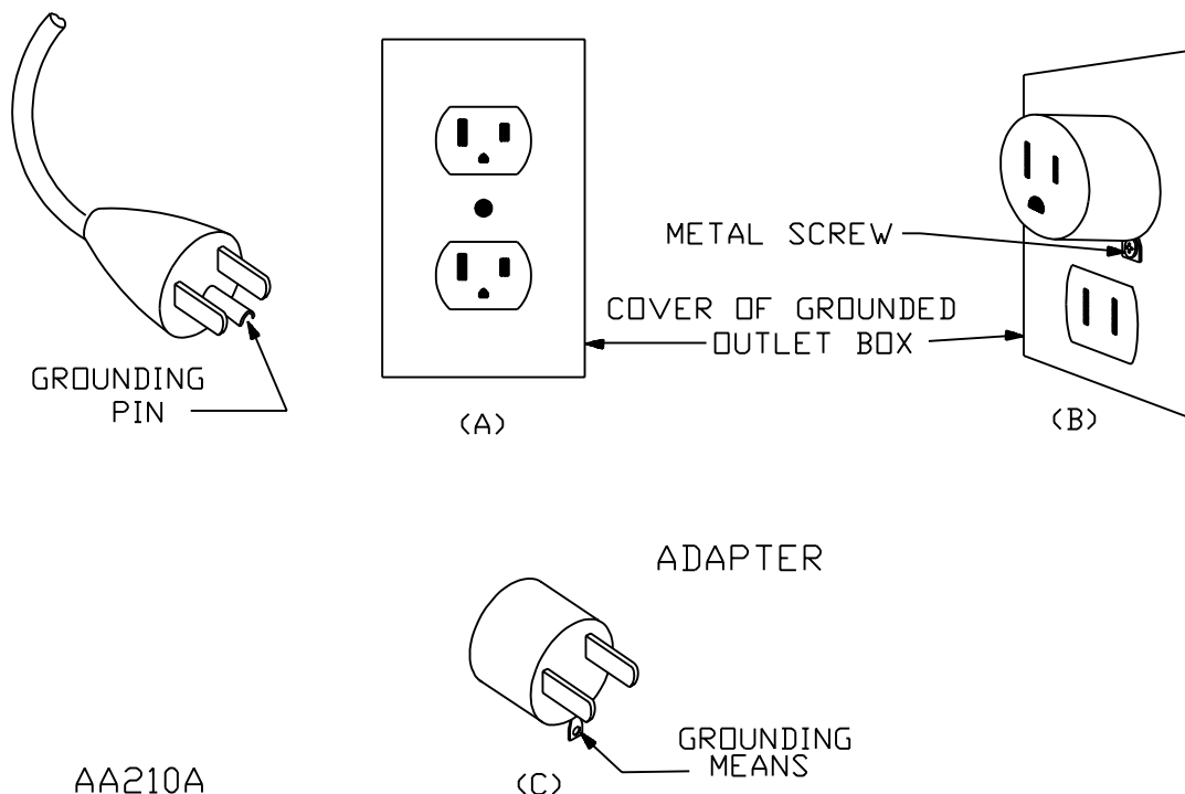
Figure SA27.1 Grounding method
