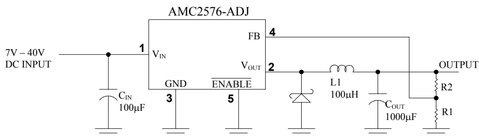
Figure 2. Adjustable Output Voltage Versions
