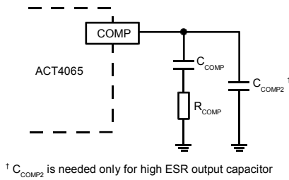
Figure 4. Stability Compensation
