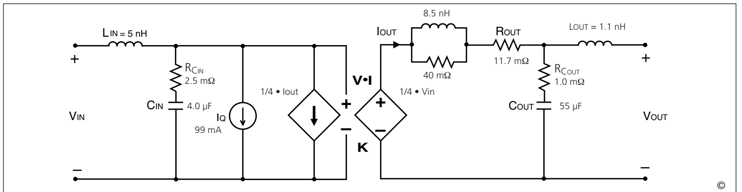
Figure 18 — This model characterizes the AC operation of the V•I Chip VTM including response to output load or input voltage transients or steady state modulations. The model enables estimates or simulations of input and output voltages under transient conditions, including response to a stepped load with or without external filtering elements.
