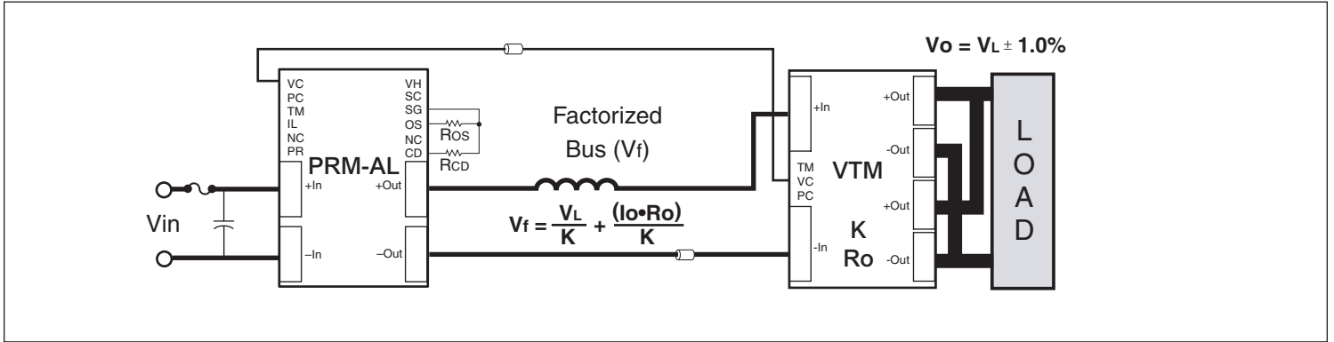
Figure 19 — The PRM controls the factorized bus voltage, Vf, in proportion to output current to compensate for the output resistance, Ro, of the VTM. The VTM output voltage is typically within 1% of the desired load voltage (VL) over all line and load conditions.
