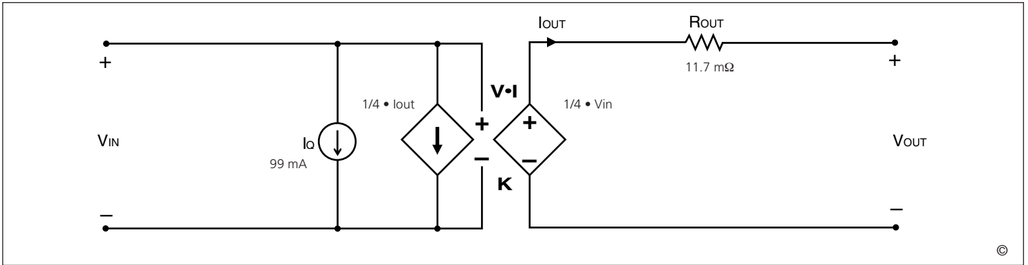
Figure 17 — This model characterizes the DC operation of the V•I Chip VTM, including the converter transfer function and its losses. The model enables estimates or simulations of output voltage as a function of input voltage and output load, as well as total converter power dissipation or heat generation.
