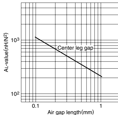
AL-value vs. Air gap length for PC40EE50.3/51/6 core (Typical)
