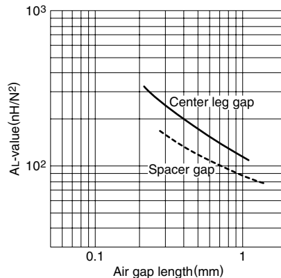
AL-value vs. Air gap length for PC40EI25 core (Typical)
