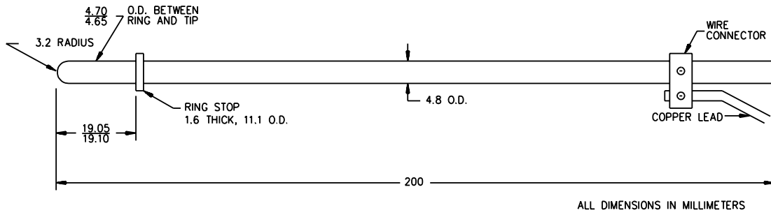
Figure 36.2 Test pin B
