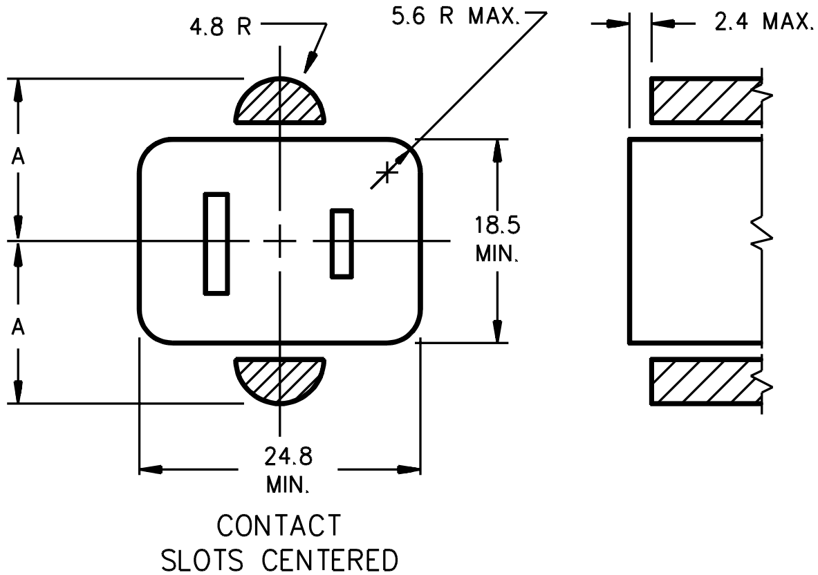
Figure 11.4 Minimum outlet face dimensions
