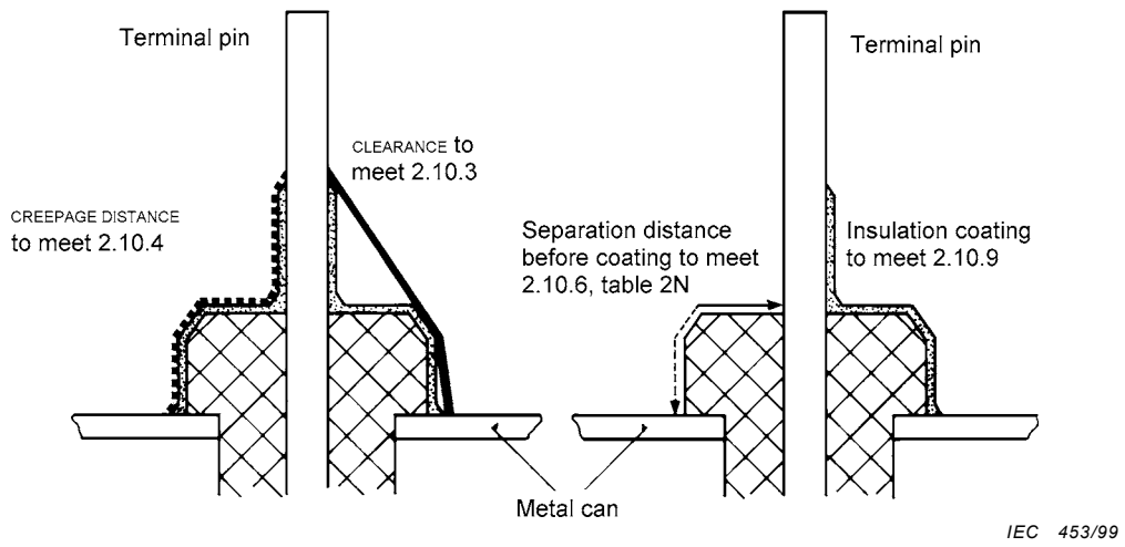
Figure F.10 – Coating around terminals
