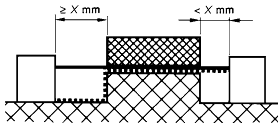
Figure F.6 – Uncemented joint with wide groove
