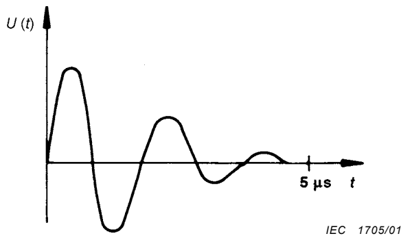
Figure S.3 – Waveforms on insulation with surge suppressors in operation
