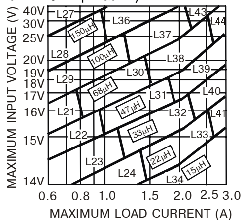
Figure 6. LM2596-12
