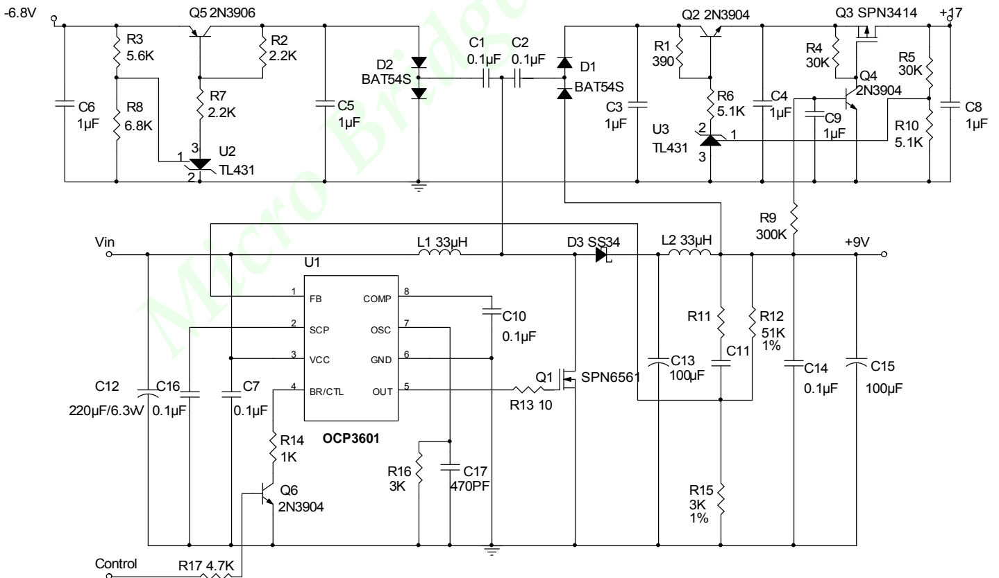
Figure17. Charge Pump DC-DC Converter Circuits
