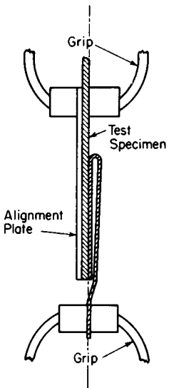
FIG. 2 Specimen Under Test
