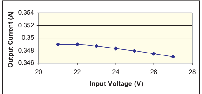
Fig. 4. Output Current vs. Input Voltage
