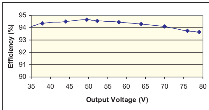
Fig. 1. Efficiency vs. Output Voltage
