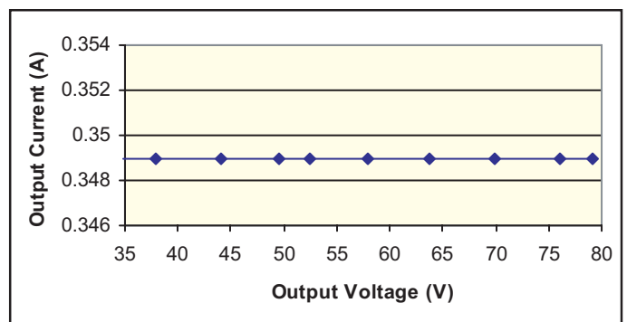
Fig. 3. Output Current vs. Output Voltage
