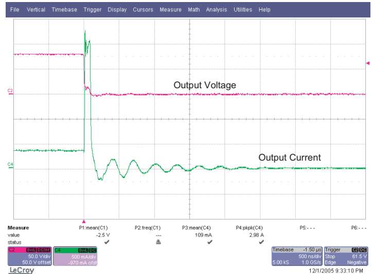
Fig. 7: Output Short Circuit Protection (500ns/div)
