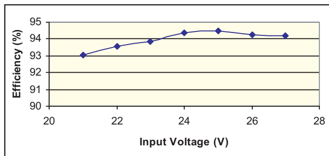
Fig. 2. Efficiency vs. Input Voltage
